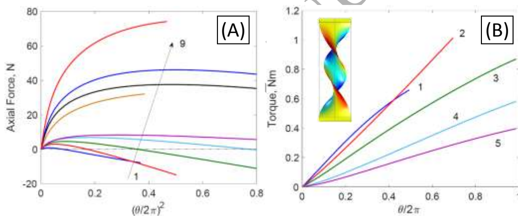
Figure 5- (A) Predicted Poynting effect utilizing a 2 nd gradient continuum model. (B) Predicted torque-twist behavior for the specimens 1 through 5 that exhibited widely contrasting Poynting behavior including reversal from positive to negative Poynting effect. Inset shows an example simulated deformed configuration at 360°.
