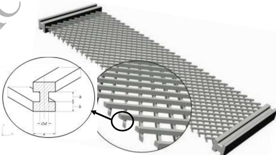
Figure 1- Schematic of continuum material point, P, with its granular microstructure and the coordinate systems x and x'
