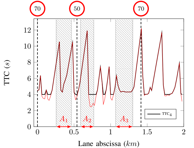
Fig. 8: Evolution of the Time To Collision parameter when adopting the proposed speed profile
