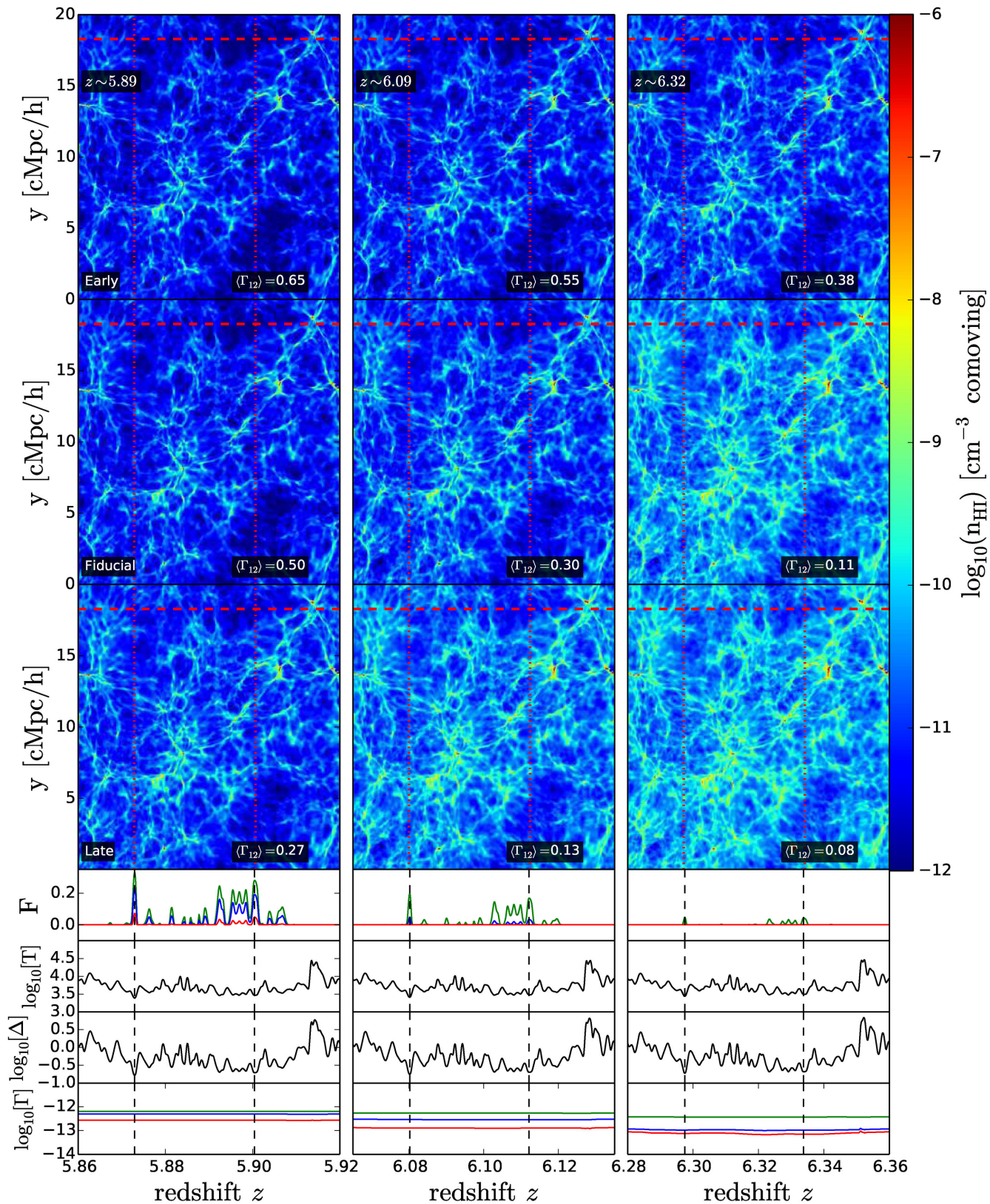
Figure 3. Example of a line of sight (shown with the red dashed horizontal lines) through the volume of our three 20 cMpc h^{-1} simulations at three different redshifts. For each model, we show the transmitted flux F , as well as the temperature T , the overdensity \Delta and the photoionization rate \Gamma in velocity space along the line of sight. The background shows the neutral hydrogen comoving density n_{\text{HI}} in the different models in a slice of 39.0625 kpc h^{-1} thickness.
