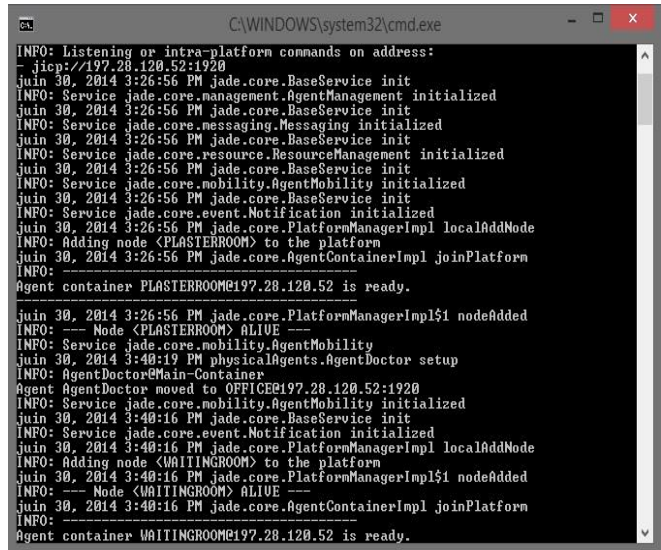
Figure 7: Agent migration
