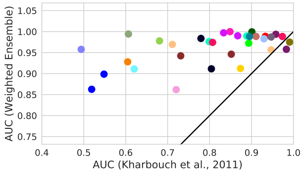
Fig. 1: Scatter plot of the ROC AUC scores (averaged) obtained on record-specific datasets of 5 s data segments using a 5-fold cross-validation. The solid black line represents the straight line joining the point (0, 0) to (1, 1).
