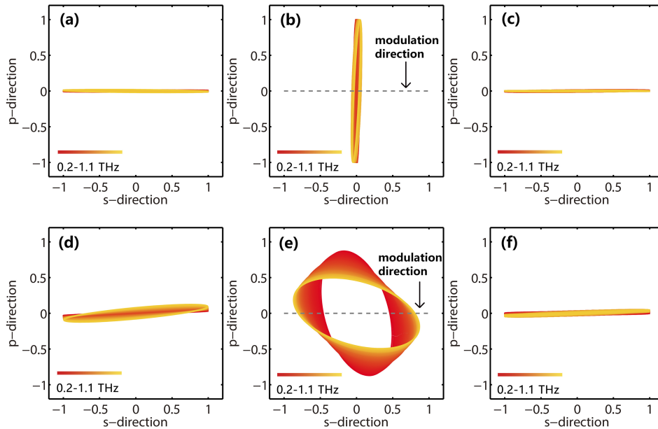
FIG. 3. The polarization states of reflected signals when the VO 2 was in the insulating state at (a) \theta = 0^\circ , (b) \theta = 47.5^\circ , and (c) \theta = 90^\circ , and the polarization states of reflected signals when the VO 2 was in the metallic state at (d) \theta = 0^\circ , (e) \theta = 47.5^\circ , and (f) \theta = 90^\circ . The dashed gray line in (b) and (e) indicates the intensity modulation in s -polarization.
