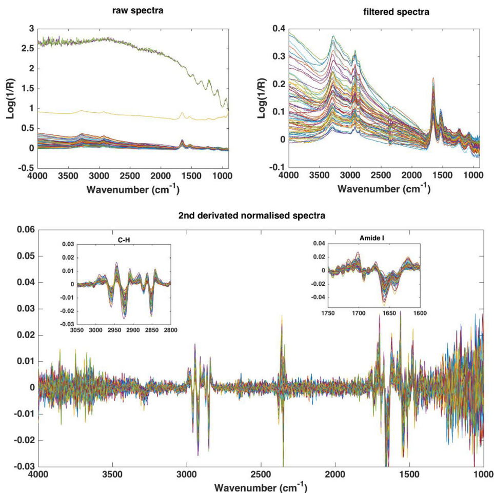
FIGURE 2. Infrared spectra preprocessing procedure. Top left, raw spectra, top right, filtered spectra (to remove background disturbed spectra), and bottom, 2nd derivative Savitzky-Golay spectra (9 pts, 2 order) and unit vector normalized. A close-up view on CH stretching and the Amide I region are shown in the bottom panel.
