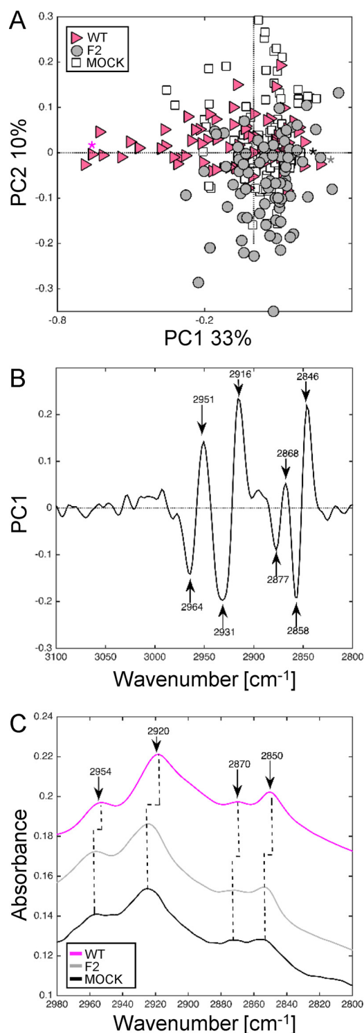
FIGURE 8. Synchrotron IR microspectroscopy comparison of mock, WT, and F2-infected U937 cells at 8 h post-infection within the CH region. A, score plot of PCA from the 3100–2800 \text{cm}^{-1} band IR spectra. The explained variance for PC1 and PC2 is 33 and 10%, respectively. Marked data with pink triangles correspond to U937 cells infected with WT virus, gray circle to cells infected with F2 virus, and white square to mock-infected cells. B, loading plot linking the variable space and principal component subspace (PC1). PCA score plots show that the WT and F2-mock groups separate along PC1. C, mean IR spectra of mock-infected cells (black line), WT (pink line), and F2-infected cells (gray line) at 8 h post-infection in the 2980–2800 \text{cm}^{-1} range. A shift for the principal peaks corresponding to CH 2 -CH 3 stretching (2954, 2920, and 2850 \text{cm}^{-1} ) associated to perturbation of membrane fluidity was observed for WT-infected cells spectra compared with mock and F2-infected cells. PC, principal component.
