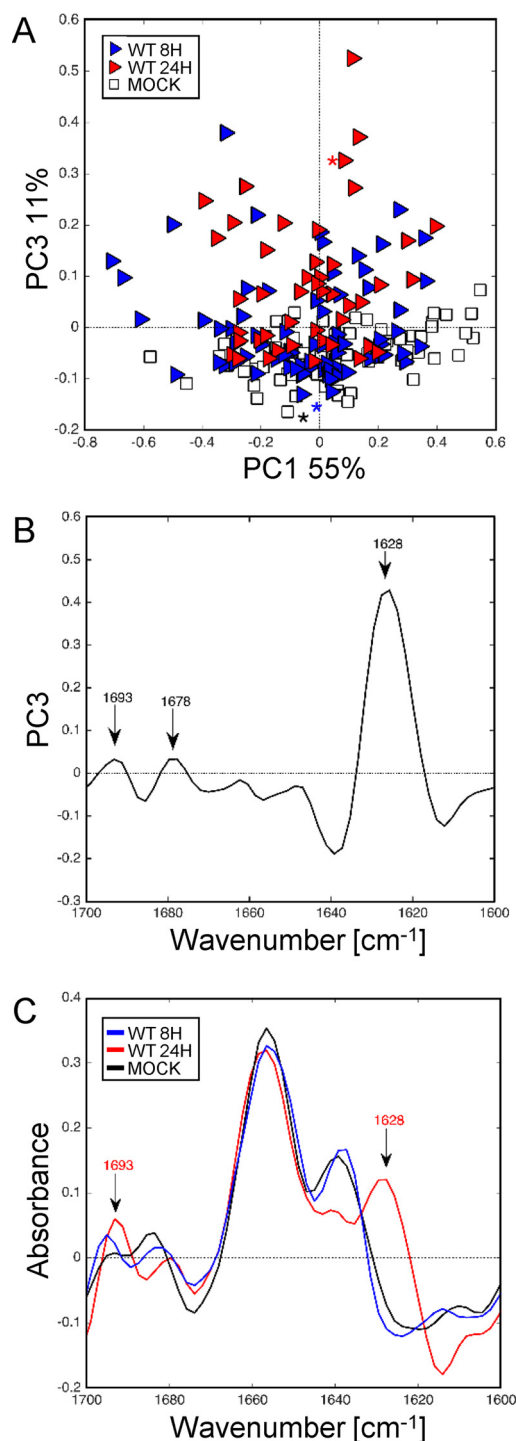
FIGURE 4. Synchrotron IR microspectroscopy comparison between the secondary structure content of mock and WT-infected U937 cells at 8 and 24 h post-infection within the amide I region. A , score plot of PCA from the 1700–1600 cm -1 band IR spectra. The explained variance for PC1 and PC3 is 55 and 11%, respectively. Marked data with the white square corresponds to mock-infected cells and blue and red triangles correspond to cells infected with WT virus at 8 and 24 h post-infection, respectively. B , loading plot linking the variable space and principal component subspace (PC3). PCA score plots show that the WT and mock groups separate along PC3. Compared with the mock group, WT groups show higher IR intensity at 1628–1693 cm -1 bands attributed to aggregated \beta -sheet structures. C , marked points second derivative spectra: mock-infected cells ( black line ) and WT-infected cells at 8 ( blue line ) and 24 h ( red line ) post-infection in the range 1700–1600 cm -1 . A progressive shift from 1643 cm -1 (unordered \beta -sheet structure) to 1628 cm -1 was observed in a time-dependent manner for WT-infected cells 2nd derivative spectra compared with mock-infected cells. PC , principal component.
