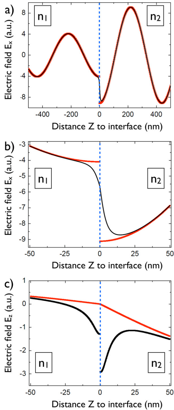
Figure A1. (a) X -component of the electric field associated with a 100 keV electron incident perpendicularly on a vacuum ( n_2 )/ \text{SiO}_2 ( n_1 ) interface calculated at 10 nm from the electron trajectory. (b) Same in a small region around the interface. (c) Z -component of the electric field associated with a 100 keV electron incident on vacuum ( n_2 )/ \text{SiO}_2 ( n_1 ) interface.
