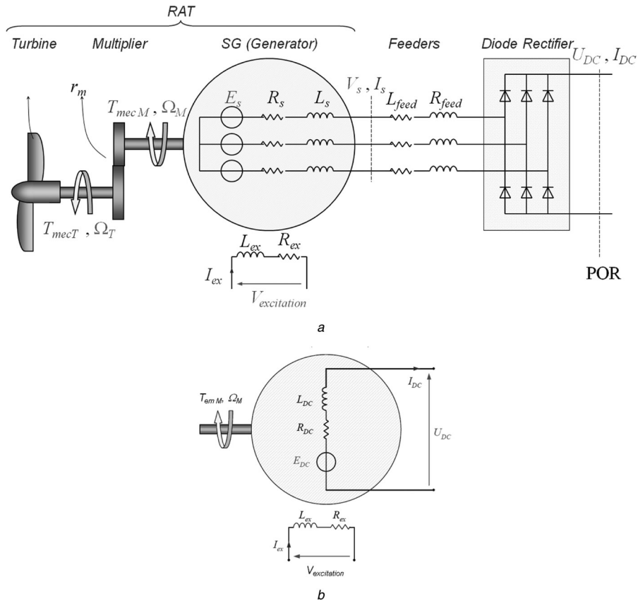
Fig. 4 Electrical scheme and its equivalent DC circuit
