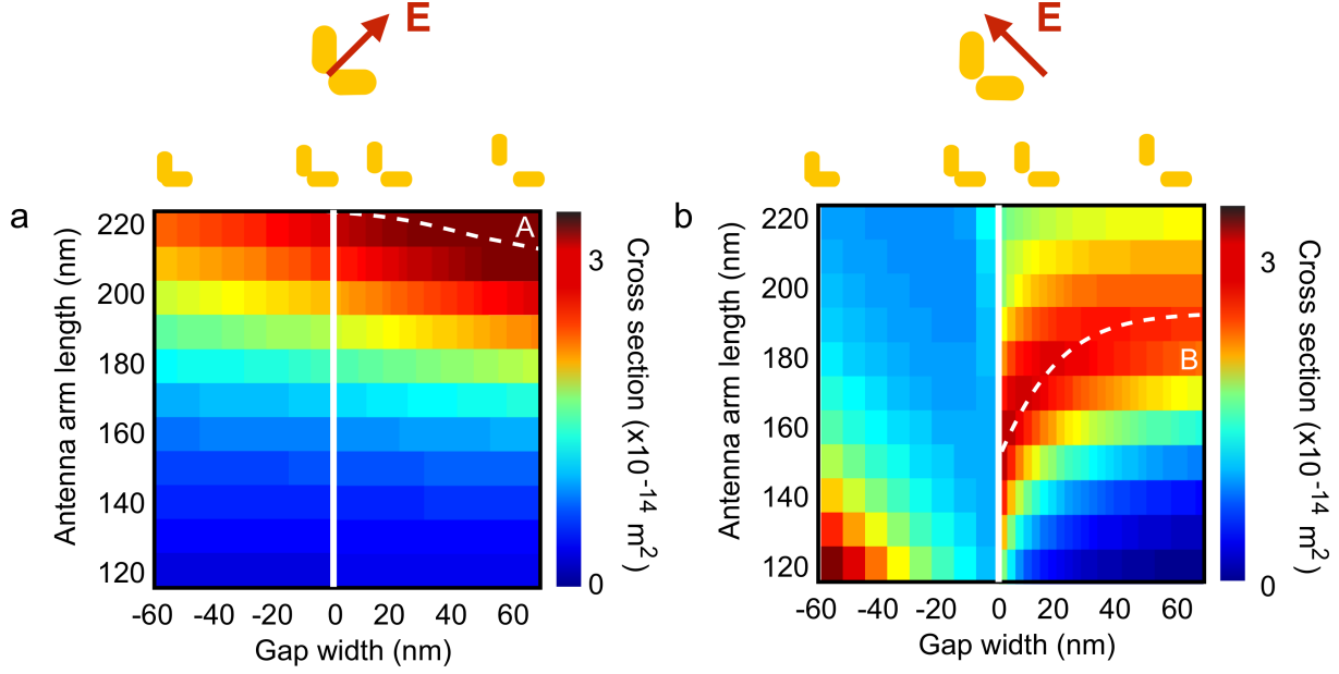
Figure S4: (color online) Map of antenna absorption cross section at \lambda_{exc} = 900 nm, as a function of antenna length L and gap width G . Dashed lines are guides to the eye indicating spectral positions of anti-bonding (A) and bonding (B) resonances.
