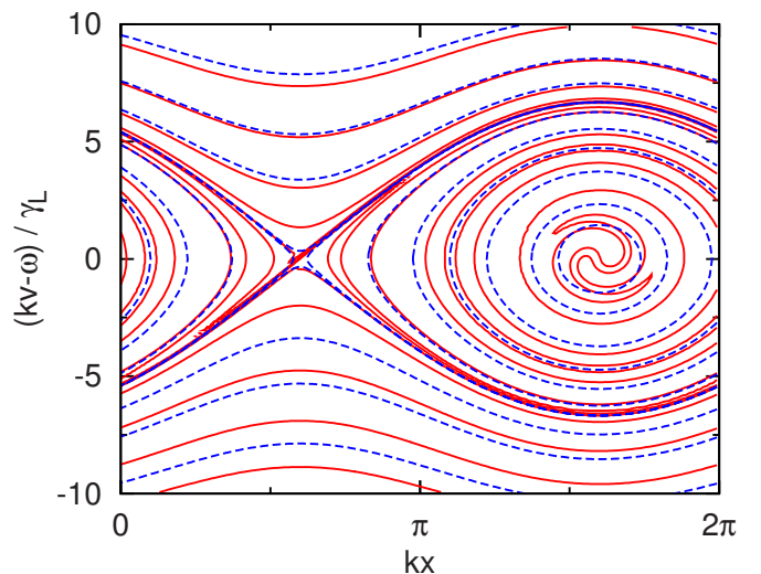
FIG. 2. (Color online) Contour plot of the time-asymptotic distribution function (solid curves) and constant energy curves (dashed curves) for the same parameters as Fig. 1.
