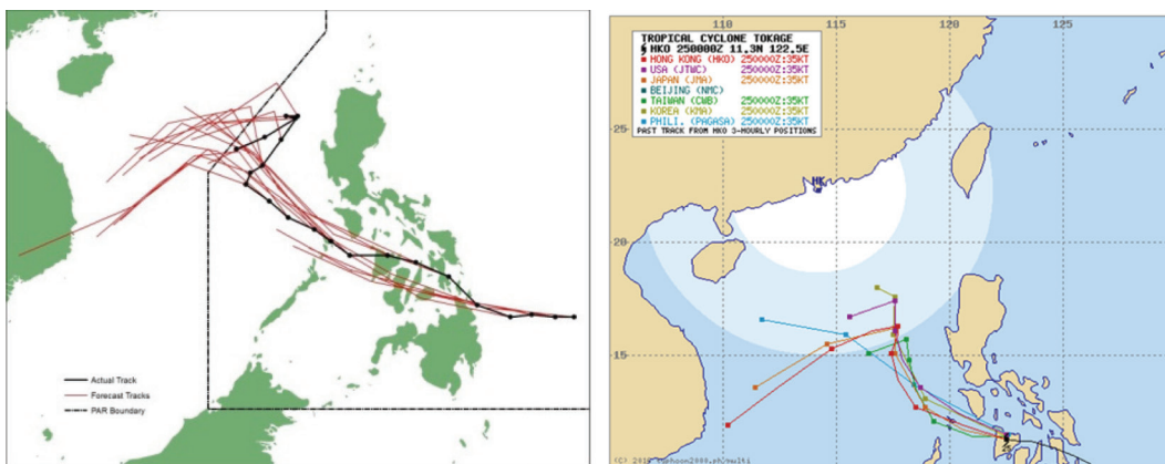
FIG. 10. (Left) 3-day forecast tracks issued by PAGASA through the lifespan of Tropical Storm Tokage. (Right) Forecast tracks of various TC warning centers at 0000 UTC 25 November.
