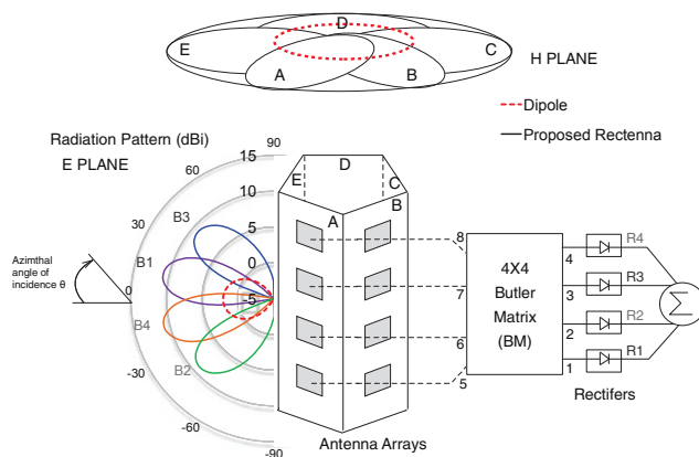
Fig. 1. Schema of the beam forming based RF energy harvester and its radiation pattern in the E plane and H plane of a linearly polarized radiation. The radiation pattern is compared to the radiation pattern of an omnidirectional dipole antenna.
