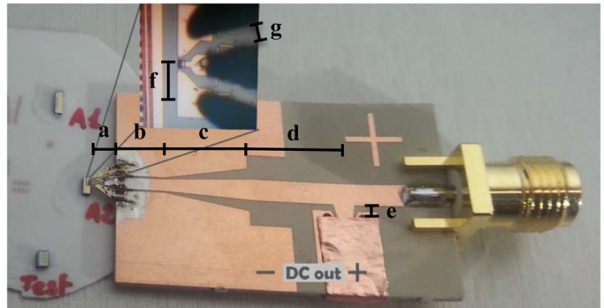
Fig. 13. Photograph of the rectifier circuit using a backward diode. The matching network was built and integrated with an in-house GSG probe used to interface with the diode pads (inset). a = 83 mil, b = 170 mil, c = 300 mil, d = 333 mil, e = 25 mil, f = 100 \mu\text{m} , g = 2 mil. Width of the line in d = 75 mil, width of the line in b = 42 mil ( 6 mil separation between line and ground).
