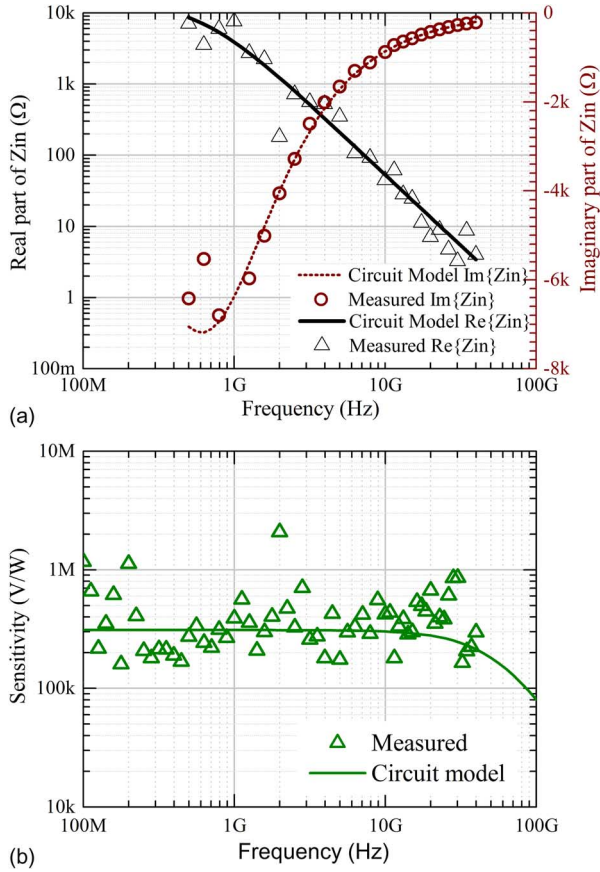
Fig. 6. Comparison between measured and modeled backward diode RF characteristics at -30 dBm. (a) Input impedance, Z_{in} , real and imaginary components. (b) Voltage sensitivity; the simulation has been projected to 100 GHz.
