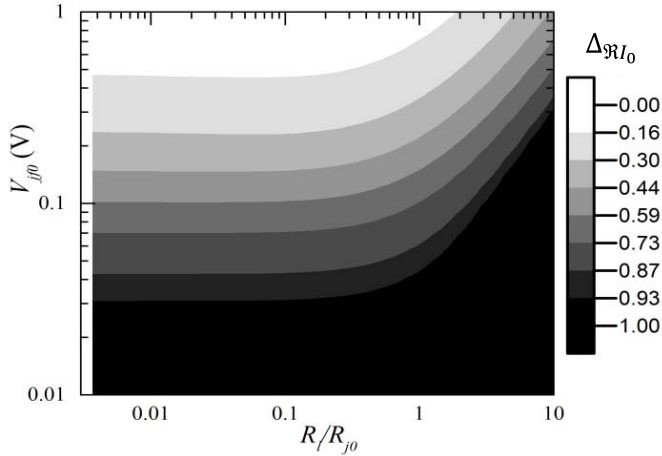
Fig. 6. \Delta_{\mathcal{R}} contours for a theoretical diode model with infinite breakdown voltage. Curves were generated using the SMS7630 diode parameters.
