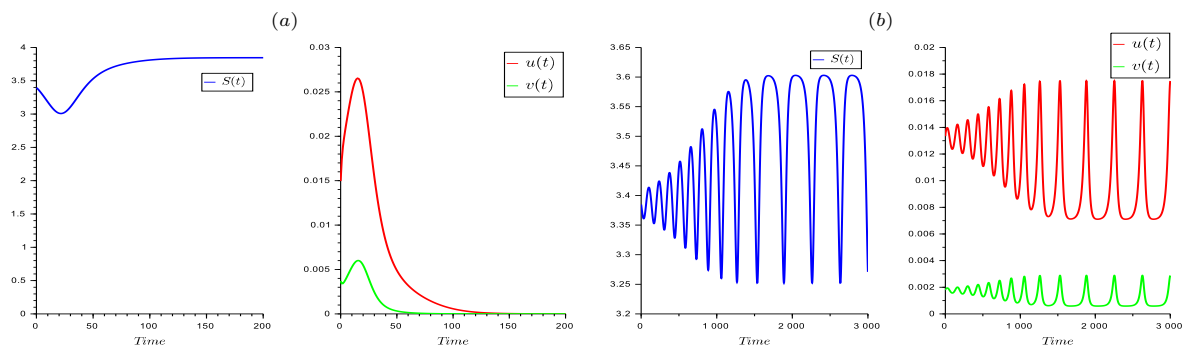
FIG. 7. Case S_{in} = 3.846 \in ]S_{in}^2, S_{in}^{h_1}[ : bi-stability with convergence either to E_0 (a) or limit cycle when the oscillations are sustained (b).
