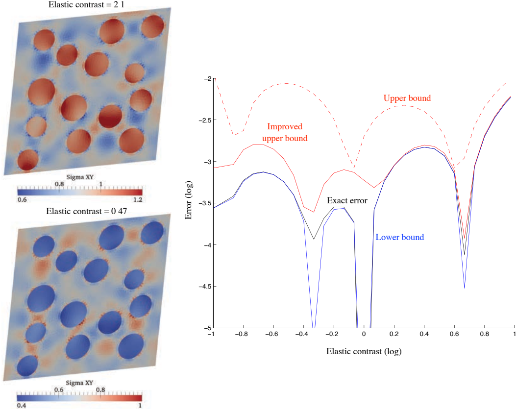
Fig. 1 – Error estimation for a Galerkin-POD reduced order model applied to the homogenisation of a particulate composite material.
