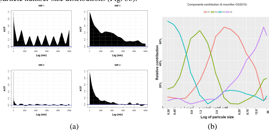
Fig 3. Autocorrelation function (ACF) of the four NMF components (a) and their relative contribution according to size particles diameter.
