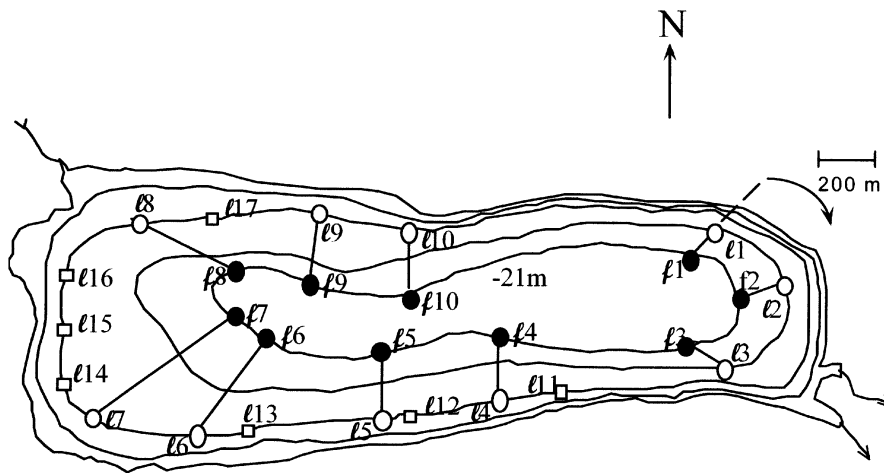
Fig. 2. Lake Châlain : location of the 27 sampling sites on the isobaths. nℓ = 17 at Zℓ, n f = 10 at Z f , Zℓ = 2m, Z f = 21 m. o : ℓ 1 to ℓ 10, on transects at Zℓ, • : f 1 to f 10, on transects at Z f , □ : ℓ 11 to ℓ 17, added littoral sites.
