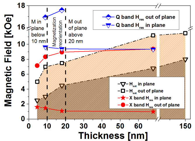
FIG. 8. (Color online) Magnetic saturation field values (in-plane and out-of-plane) and the respective resonance field values in the X-band and Q-band FMR experiment at 15 K, as a function of film thickness. Vertical dashed lines indicated the magnetization reorientation region reported in Ref. [7].
