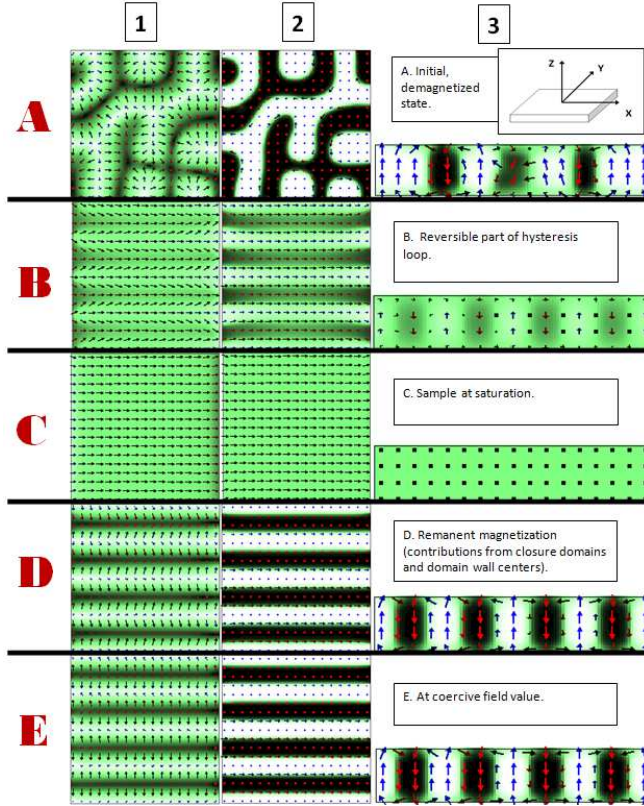
FIG. 3. (Color online) Diagrams showing magnetic moment distribution in different parts of 30 nm \text{Mn}_5\text{Ge}_3 film, computed with the use of OOMMF software package. Magnetic field applied in the film plane, rows (A,B,...E) correspond to characteristic points of hysteresis loop in Fig. 1. Columns represent different projections: [1]: Top view at sample surface, [2]: x-y cross section at half-thickness and [3]: y-z cross section. For details see the text.
