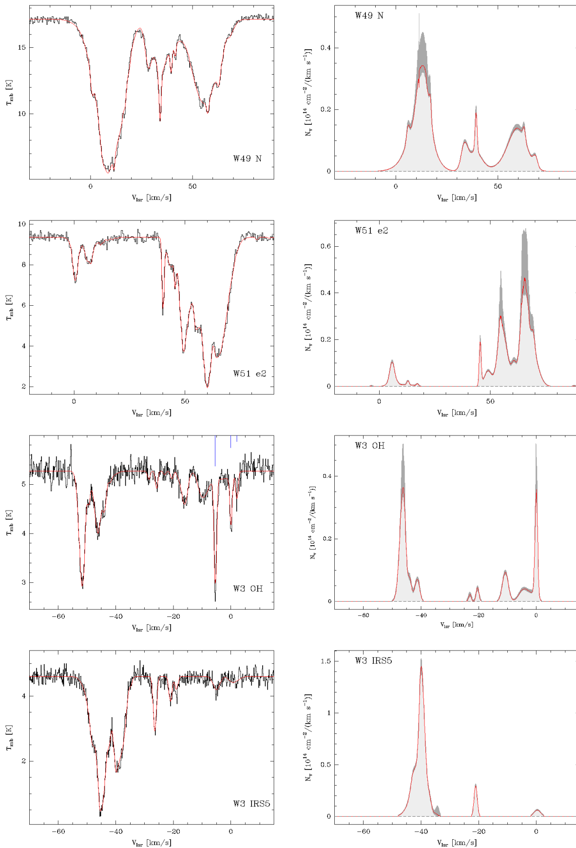
Fig. 2. CH \lambda 149 \mu\text{m} spectra (left, the reference frequency for the velocity scale given by the second HFC) and deduced column density profiles (right) for (from top to bottom): W49 N, W51 e2, W3(OH), W3 IRS5. The blue markers in the W3(OH) spectrum show the hyperfine splitting and weights). The median column densities are indicated by the red lines. The dark-gray-shadowed profiles indicate the (-\sigma_-, +\sigma_+) limits, that is, 84.13% confidence, assuming a 5% error in the continuum level.
