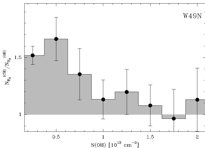
Fig. 7. As in Fig. 6, but using OH as \text{H}_2 proxy instead of HF. The ordinate shows the ratio between \text{H}_2 column densities derived from CH and those derived from OH (assuming an OH/ \text{H}_2 abundance of 10^{-7} ).
