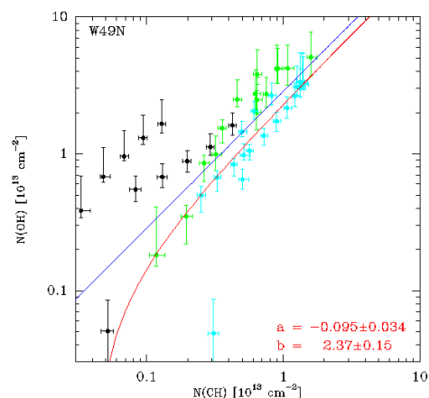
Fig. 5. Correlation between OH and CH column densities towards W49 N. The blue line is for a N(\text{OH})/N(\text{H}_2) ratio of 10^{-7} . The red line shows the weighted linear regression, the resulting OH/CH abundance ratio is given in the lower-right corner. Velocity bins for the column densities and color-codes are as in Fig. 3.
