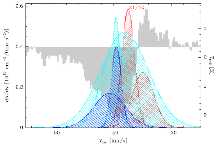
Fig. 9. Breakup of CH components observed around W3 IRS5. Red: dN/dv for the two hot core components (scaled down by a factor of 50). Cyan: Same for the three common-envelope components. Blue: Cold foreground components. The gray histogram shows the P Cygni profile of the HF ground-state transition ( J = 1 \rightarrow 0 , archival HIFI data, PRISMAS key science project). For details see text and Table 3.
