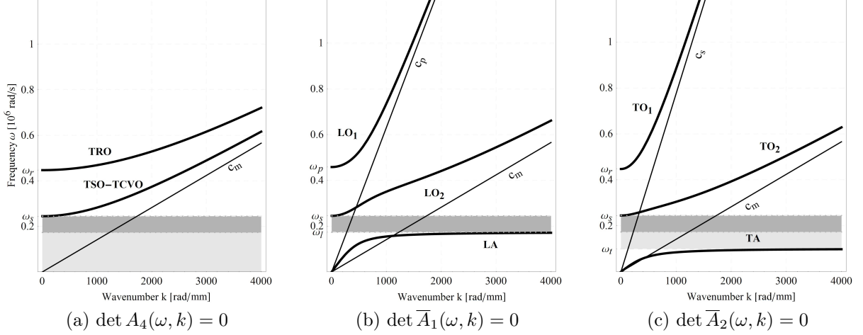
Figure 1: Dispersion relations \omega = \omega(k) [20] for the relaxed micromorphic model with non-vanishing Cosserat couple modulus \mu_c > 0 . Uncoupled waves (a), longitudinal waves (b) and transverse waves (c). TRO: transverse rotational optic, TSO: transverse shear optic, TCVO: transverse constant-volume optic, LA: longitudinal acoustic, LO 1 -LO 2 : 1 st and 2 nd longitudinal optic, TA: transverse acoustic, TO 1 -TO 2 : 1 st and 2 nd transverse optic.
