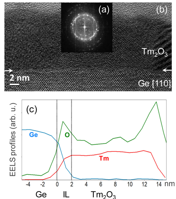
FIG. 4. Electron diffraction pattern (a), HRTEM image (b), and derived EELS elemental profiles across the interface (c), for 10 nm (nominal) \text{Tm}_2\text{O}_3 on Ge (white arrows in (b) help to locate the interface).
