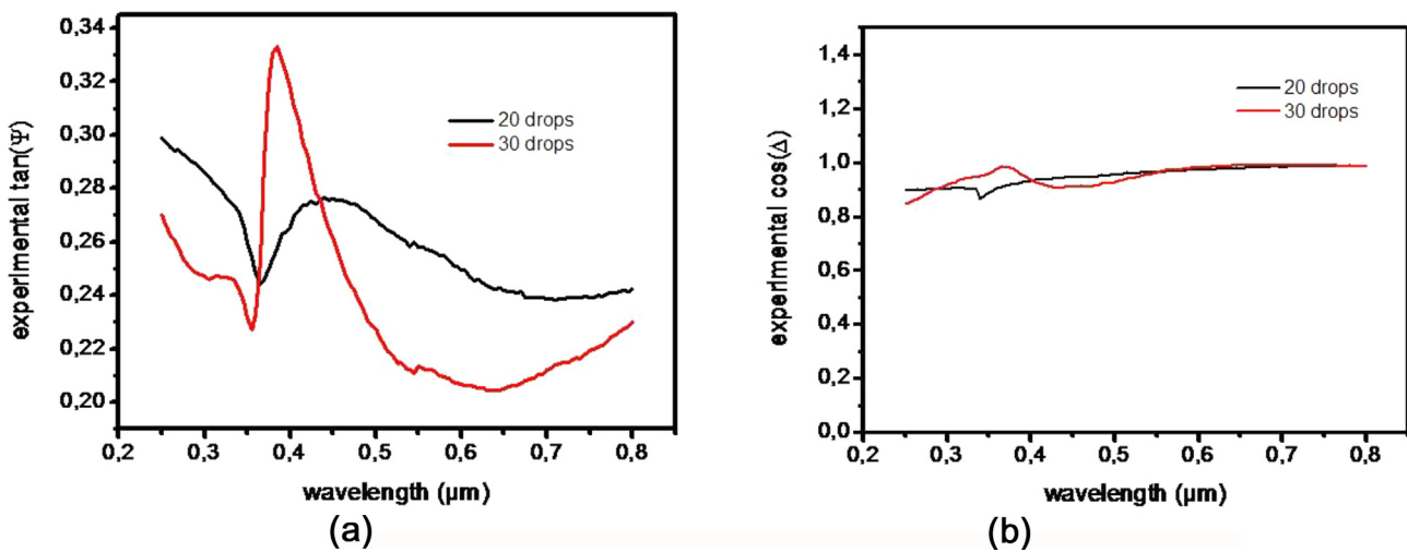
Fig. 6. Plot of \tan(\psi) (a) and \cos(\Delta) (b) of ZnO microdropped nanofilms.
