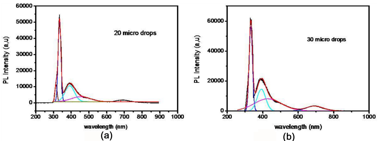
Fig. 14. Room temperature PL spectra of ZnO microdropped thin films.
