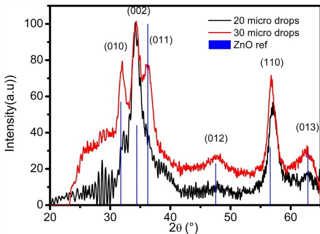
Fig. 1. DRX spectra of ZnO nanofilms.
