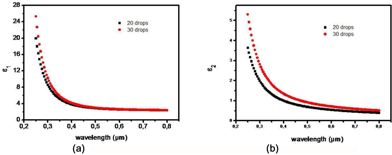
Fig. 7. Plot of \epsilon_1 (a) and \epsilon_2 (b).
