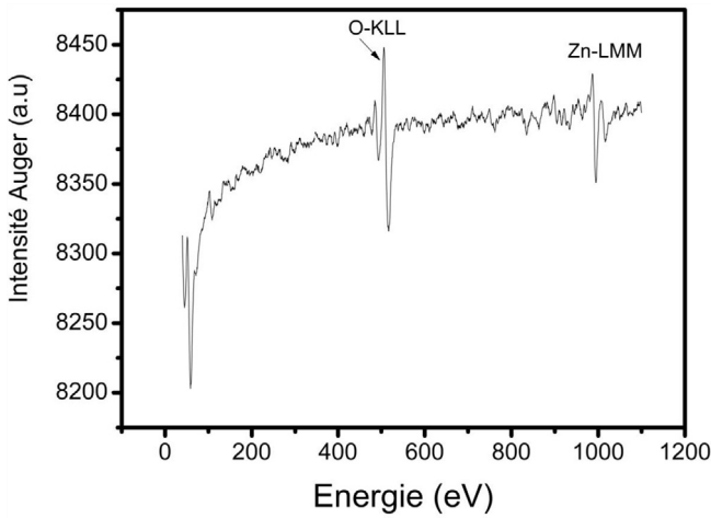
Fig. 4. Auger spectra of ZnO nanofilms after Ar + bombardment.
