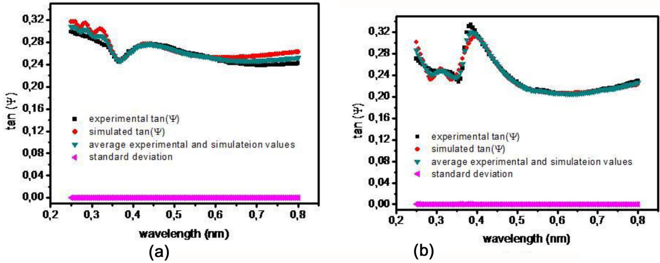
Fig. 10. Experimental, simulated, average experimental and standard deviation plot of \tan(\Psi) : (a) for sample #S1, (b) for #S2.
