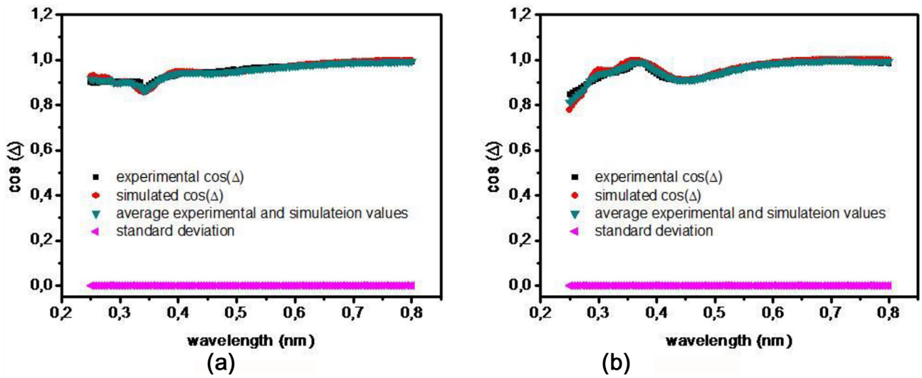
Fig. 11. Experimental, simulated, average experimental and standard deviation plot of \cos(\Delta) : (a) for sample #S1, (b) for #S2.
