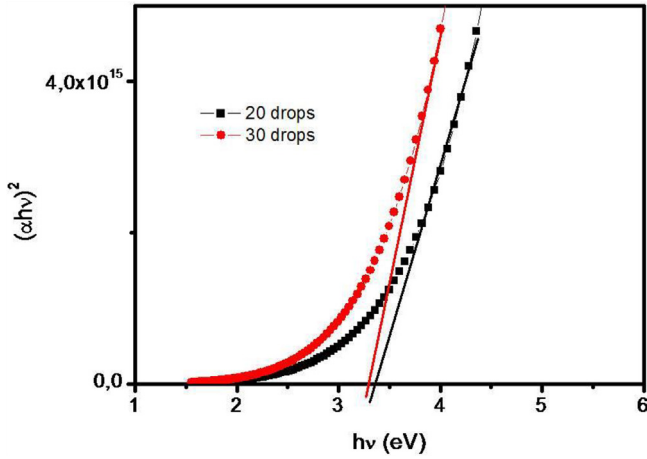
Fig. 13. Plot of (\alpha hv)^2 versus photon energy of ZnO microdropped thin films.
