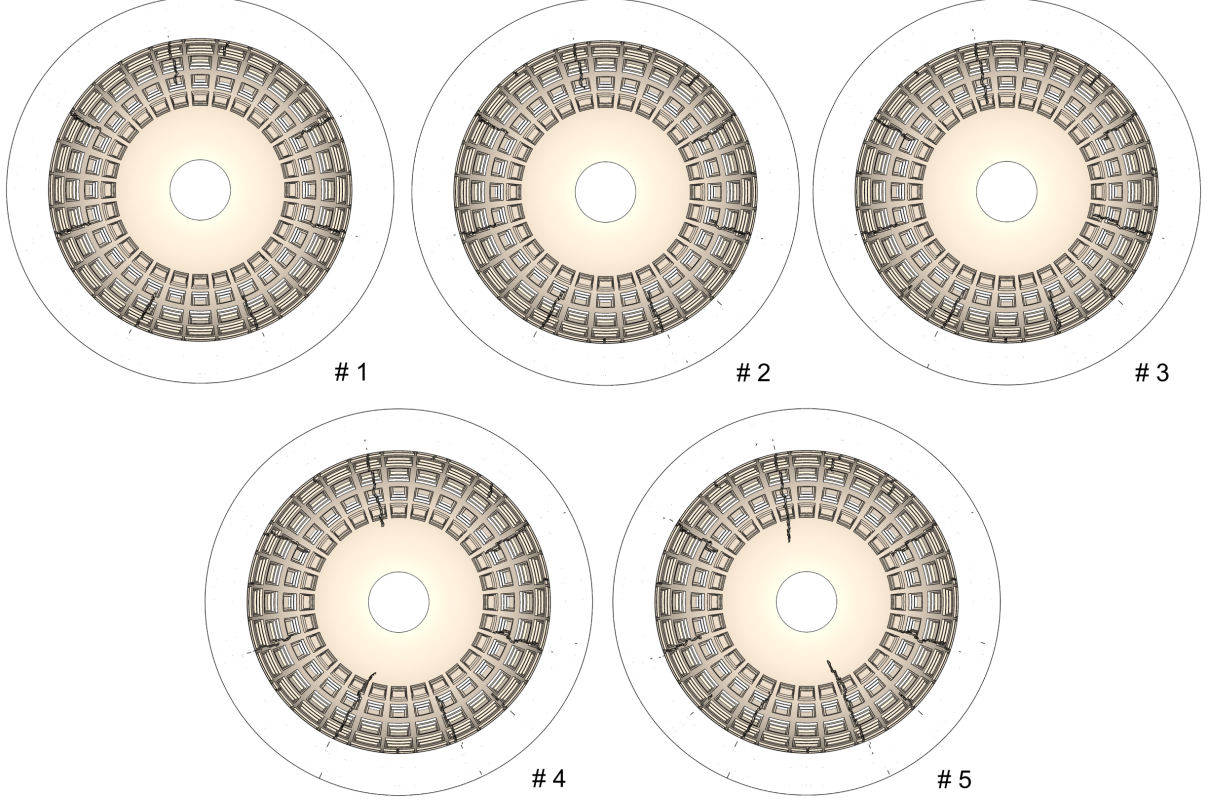
Figure 6: Crack patterns at the end of the calculations for the different volumetric strain to thermal expansion coefficient ratios, as defined in Table 2.
