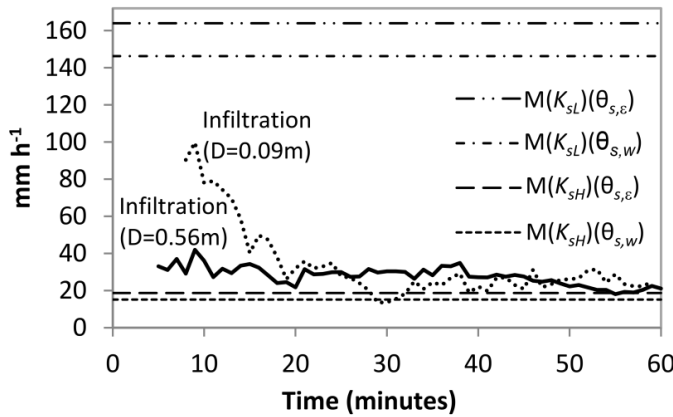
Figure 4. Comparison between the mean K_s values obtained by pouring water into the cylinder from two different heights (L and H runs) and considering different saturated soil water content values ( \theta_{s,w} and \theta_{s,\varepsilon} ), and mean infiltration rates of the rainfall simulation experiments for the 0.09 m and 0.56 m diameter plots
