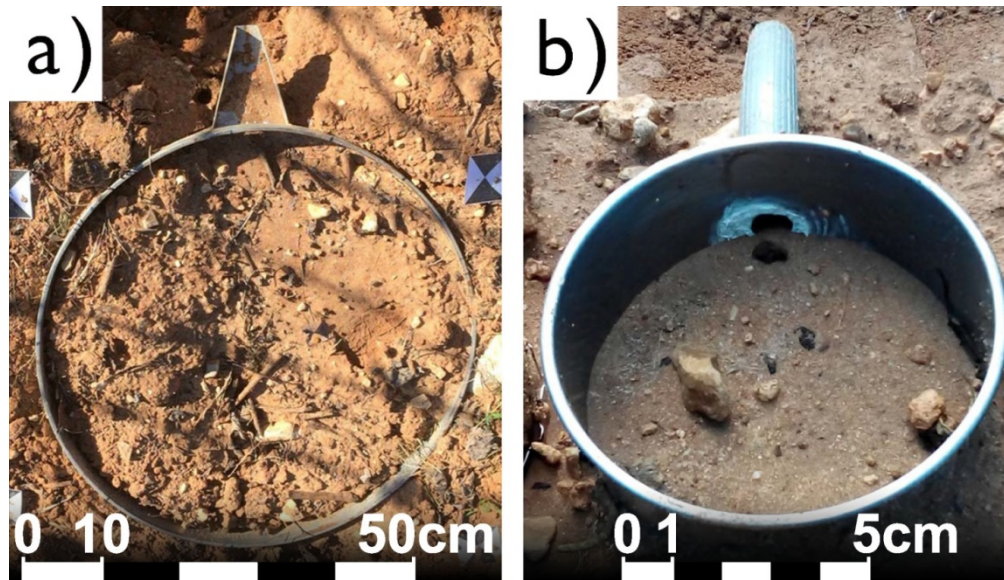
Figure 1. View of the a) 0.56 m and b) 0.09 m diameter plots
