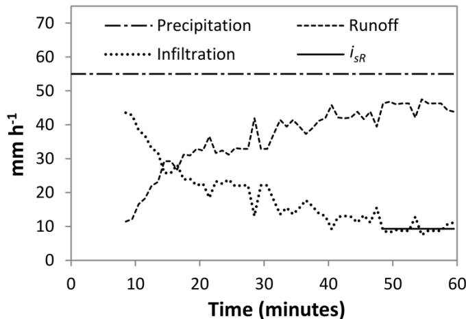
Figure 2. Illustrative example of a 1-hour simulated rainfall on a 0.56 m diameter plot at 55 mm h -1 rainfall intensity. The infiltration curve was drawn by subtracting the runoff rate from the intensity. The experimental steady-state infiltration rate, i_{sR} (9.3 mm h -1 ), was estimated considering the last thirteen data points
