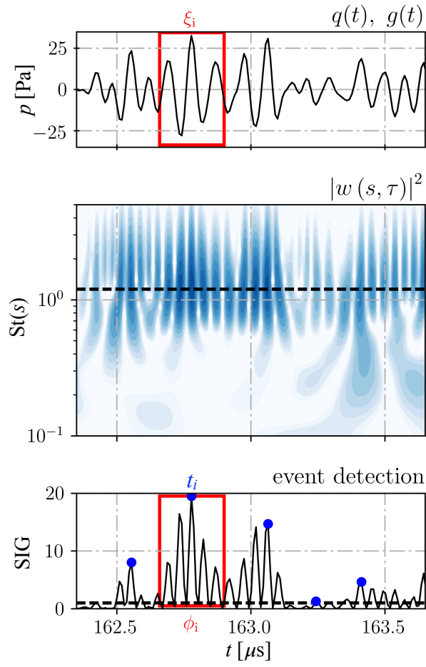
Figure 1: Wavelet transform procedure: (top) initial pressure signal q(t) ; (central) resulting wavelet power and scale of interest in dashed line ; (bottom) filtered detected events at times t_i
