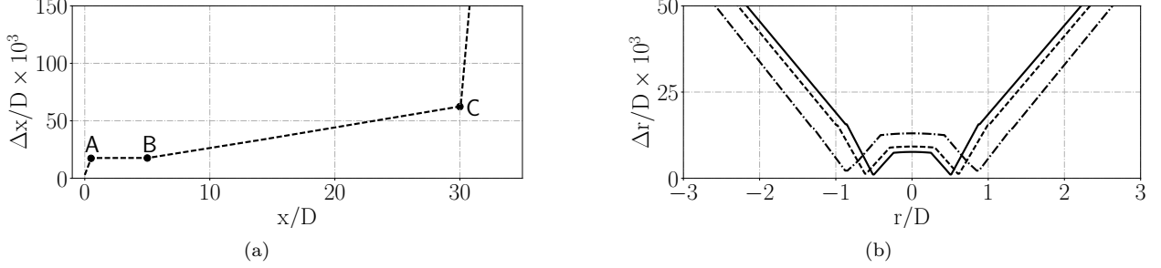
Figure 5: Mesh size (a) along the axis of the jet and (b) along gridlines perpendicular to the jet axis at x/D = 0 (solid), x/D = 5 (dashed), x/D = 10 (dash-dotted)
