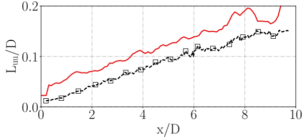
Figure 23: Axial turbulence length-scale at LIPLINE( r/D = 0.5 ). Legends: \text{-}\square\text{-} LMFA experiment [46], \text{---} LES
