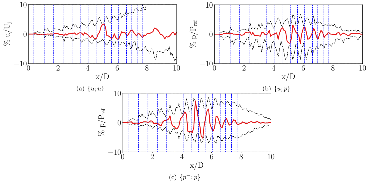
Figure 13: Cross-conditioning at AXIS ( x/D = 5 ) of axial velocity and pressure variables using different localization variables. The dashed black line represents the envelope of the signature for all axial positions. The vertical dashed blue lines represent the peak of the expansion region of each shock-cell
