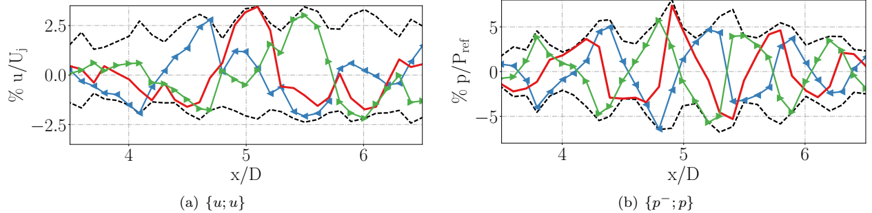
Figure 14: Cross-conditioning at AXIS ( x/D = 5 ) of (a) axial velocity u and (b) pressure p at different times. The left blue triangles ( \leftarrow ) represent the signature at \tau = -0.42D/U_j , the solid red line ( \text{---} ) at \tau = 0 and the right green triangles ( \rightarrow ) at \tau = +0.42D/U_j . The dashed line represents the envelope of the signature for all shifted times
