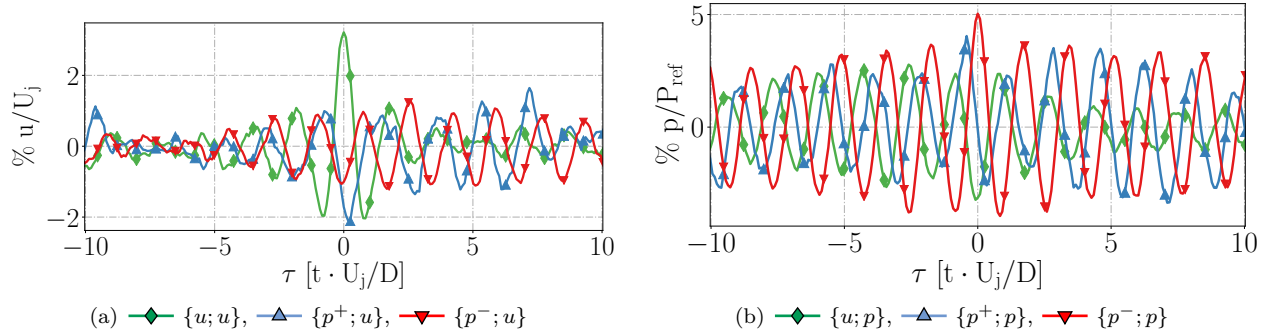
Figure 12: Signature at P0 (AXIS) of (a) u and (b) p variables
