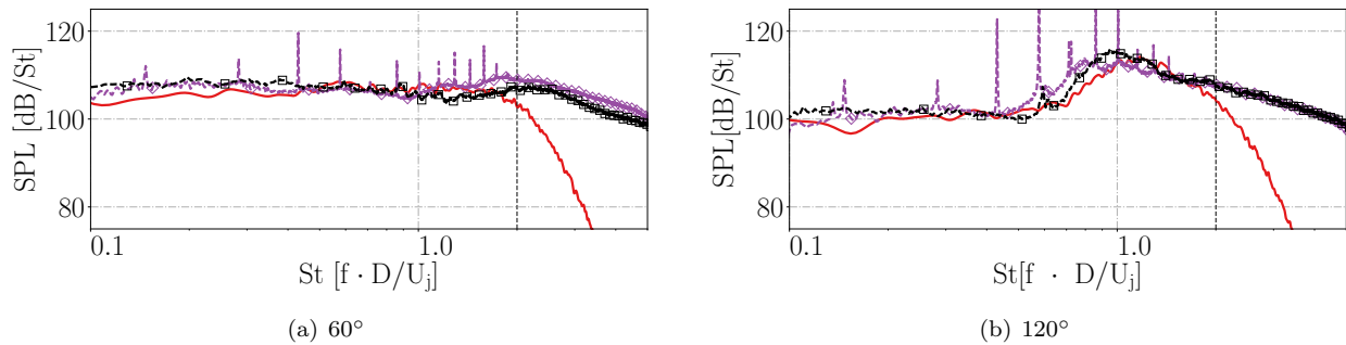
Figure 24: Far-field sound pressure level at r/D = 53 from the nozzle exit at (a) 60^\circ and (b) 120^\circ with respect to the jet direction. The vertical dashed line represents the cut-off St for the LES. Legends: \text{-}\square\text{-} LMFA experiment [46], \text{-}\diamond\text{-} experiment VKI [61] and \text{---} LES
