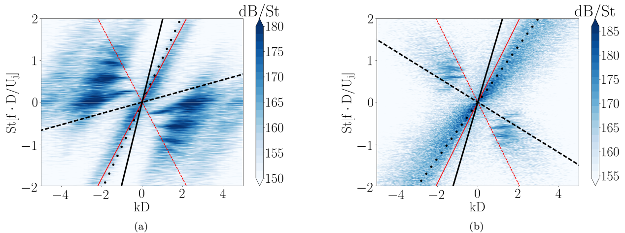
Figure 10: Frequency-wavenumber pressure energy distribution maps along the axial direction for the data set (a) AXIS and (b) LIPLINE. The dotted line depicts the mean convective velocity U_c . The thin red lines represent the acoustic speeds +a_\infty (solid) and -a_\infty (dashed). The thick lines represent U_c + a_\infty (solid) and U_c - a_\infty (dashed)
