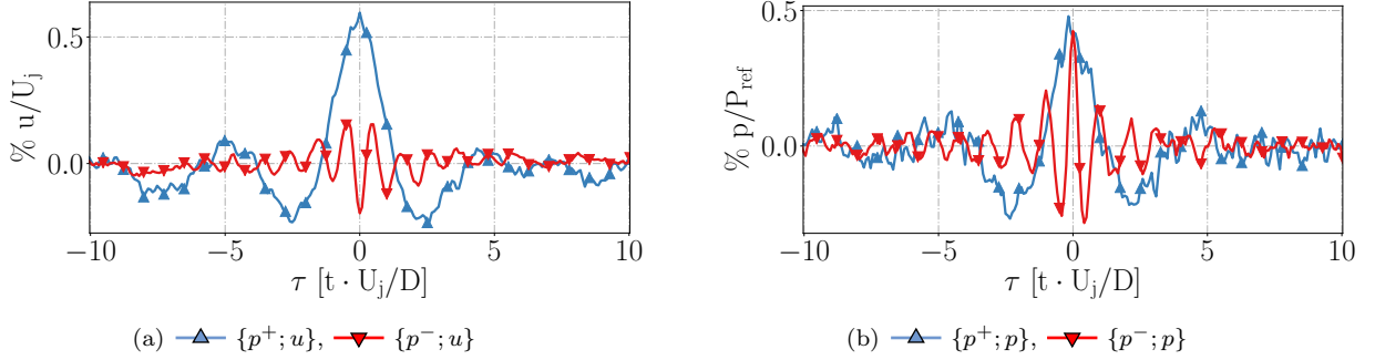
Figure 18: Signature at P2 (NEARFIELD) of (a) u and (b) p variables
