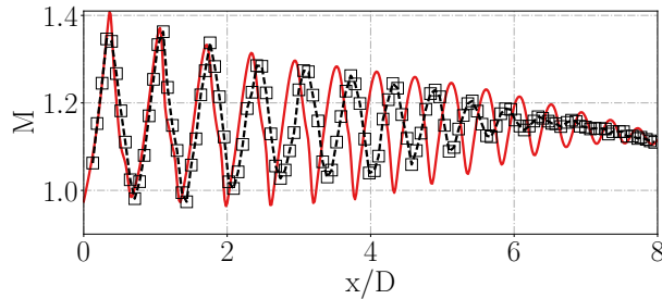
Figure 21: Mach number profile at AXIS. Legends: \text{-}\square\text{-} LMFA experiment [46] (notched nozzle), \text{---} LES
