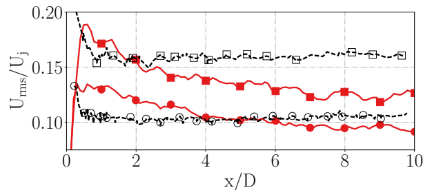
Figure 22: Turbulence levels of the axial ( U_{rms} ) and radial ( V_{rms} ) component of velocity at LIPLINE ( r/D = 0.5 ). Legends: U_{rms} \text{-}\square\text{-} and V_{rms} \text{-}\circ\text{-} from LMFA experiment [46]. U_{rms} \text{---}\square\text{---} and V_{rms} \text{---}\circ\text{---} from LES
