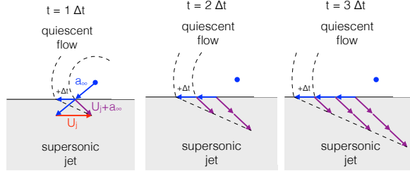
Figure 11: Evolution of a front wave traveling upstream inside a supersonic jet
