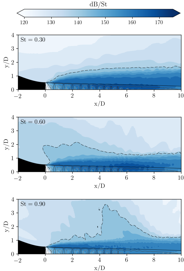
Figure 8: Average PSD maps of pressure at Strouhal numbers St = 0.3, 0.6, 0.9 , from top to bottom, respectively. The dashed line depicts the contour at 140 dB/St. The black solid lines represent the sonic line
