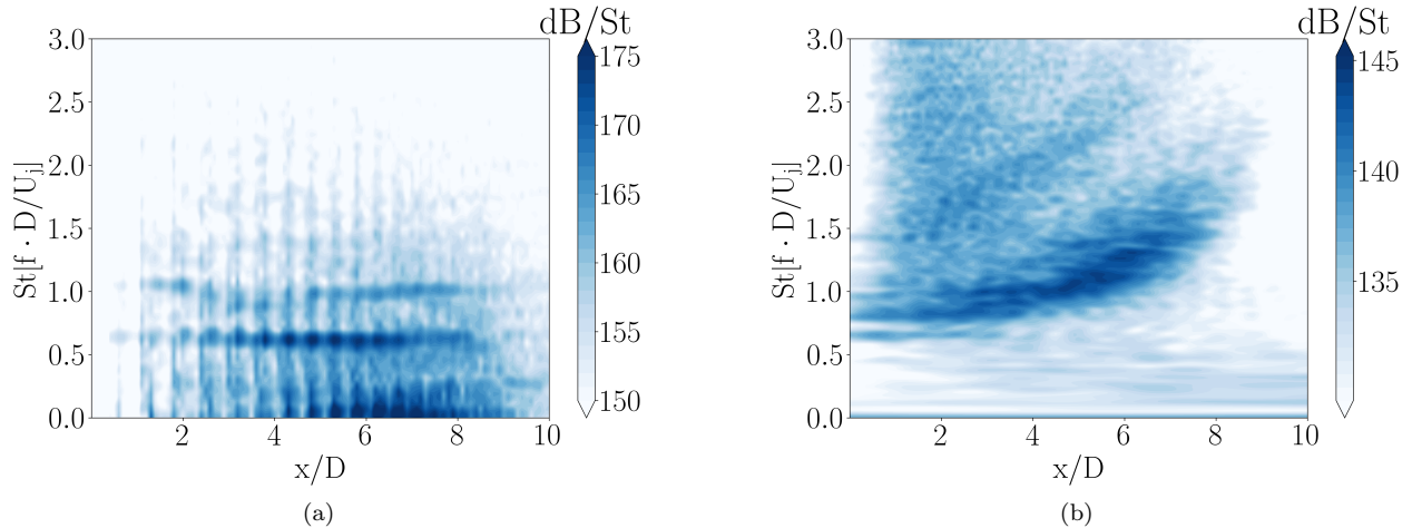
Figure 9: Frequency-space PSD maps of pressure along the axial direction for the data set (a) AXIS and (b) NEARFIELD
