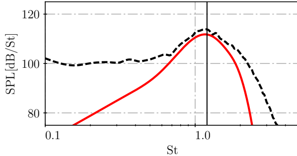
Figure 3: Far-field sound pressure level: - - - from the original pressure signal shown in Fig. 1 and — from the signature shown in Fig. 2. The vertical line depicts the scale selected for the event detection procedure
