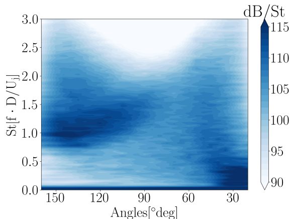
Figure 7: Far-field directivity of sound pressure level at r/D = 53 from the nozzle exit with respect to the jet direction
