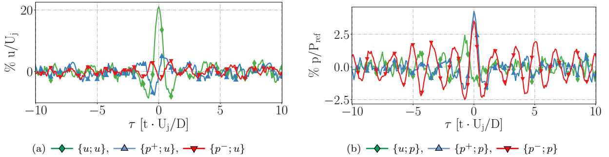
Figure 16: Signature at P1 (LIPLINE) of (a) u and (b) p variables
