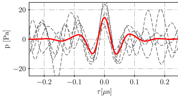
Figure 2: Example of conditional averaging (auto-conditioning) from the example shown in Fig. 1. — signature. --- windows \xi_i before averaging
