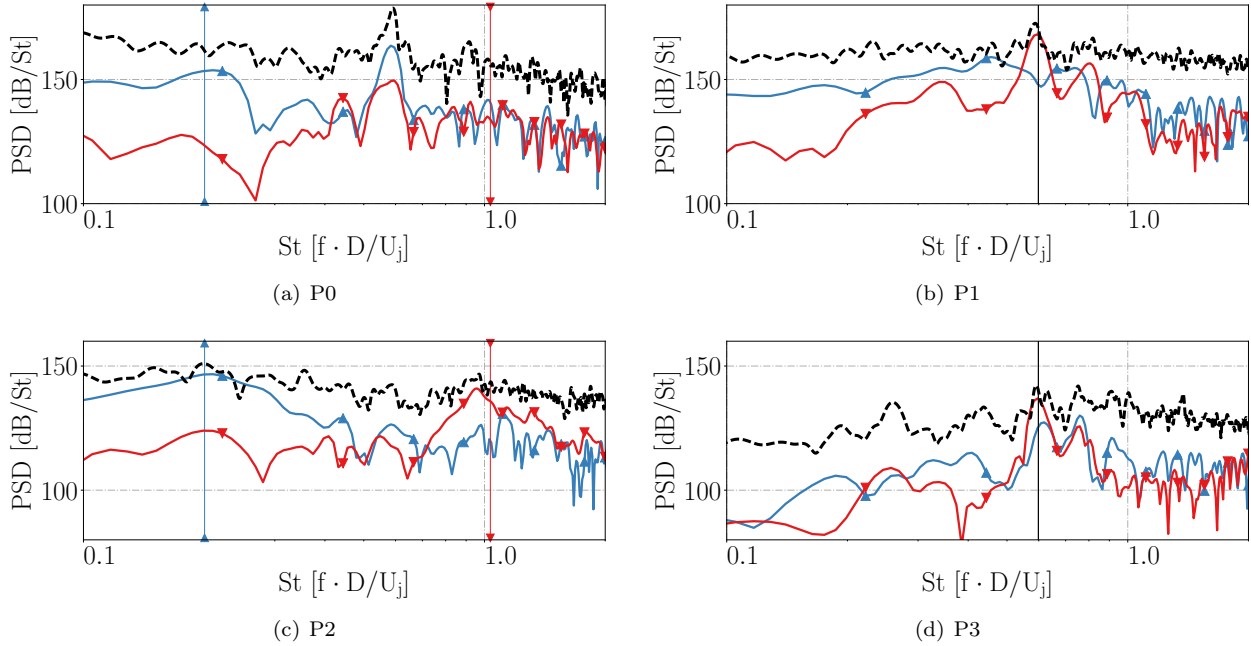
Figure 20: PSD spectra of the cross-conditioning of pressure at (a) P0, (a) P1, (a) P2 and (a) P3 computed with events detected at P1 ((b) and (d)) and P2 ((a) and (c)). --- corresponds to the PSD of the actual pressure p signal at the corresponding location, \blacktriangledown is the PSD of \{p^-; p\} , \blacktriangle is the PSD of \{p^+; p\} and the vertical lines depict the reference scales at St = 0.2, 0.6, 1.03 used in section 4.2 to detect the events
