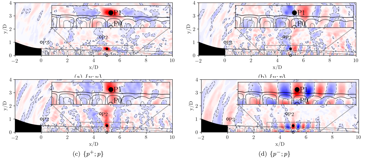
Figure 17: Normalized two-dimensional cross-conditioning maps of (a) \{u; u\} , (b) \{u; p\} , (c) \{p^+; p\} and (d) \{p^-; p\} , where the reference signal is located at P1. The results are normalized by the local standard deviation and are plotted between +1 (red contours) and -1 (blue contours). The dashed contours depict the negative regions. The black solid lines represent the Mach number contours above 1
