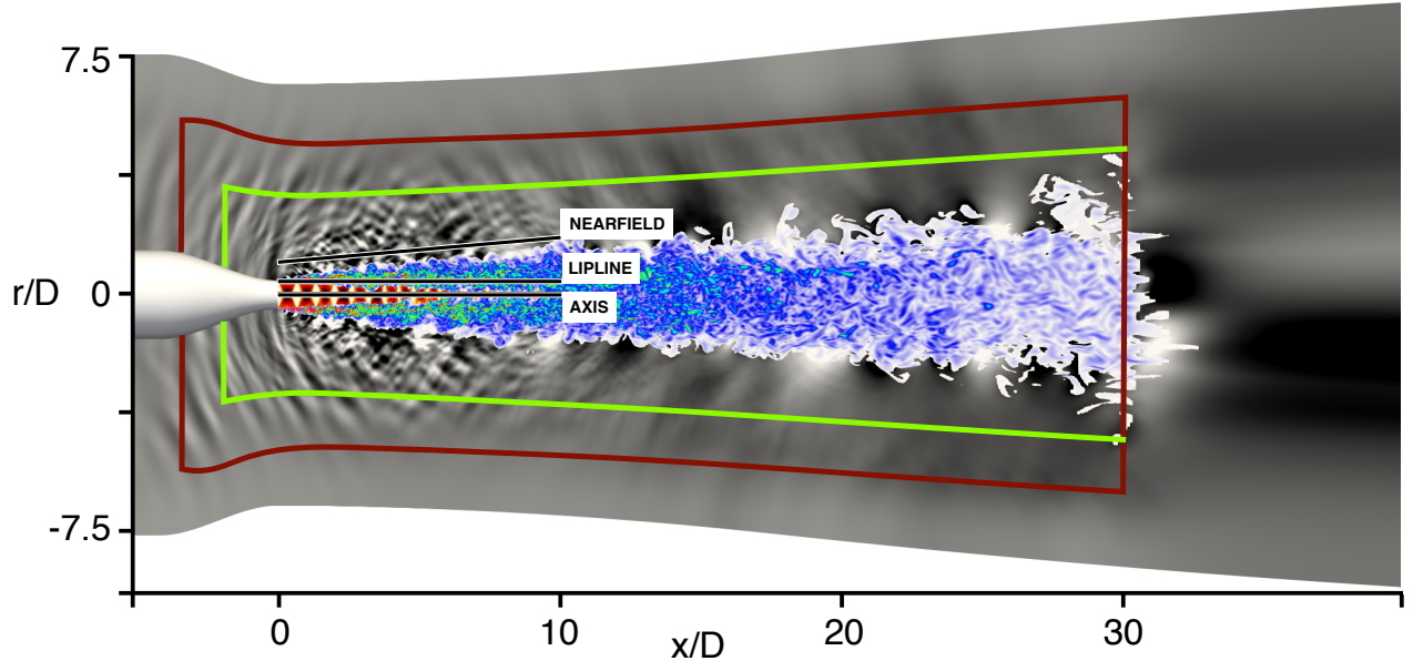
Figure 4: LES of the under-expanded jet: vorticity modulus (in color, |\Omega| \in [1.8, 320.0] \times 10^4 \text{ s}^{-1} ) and acoustic radiated pressure fluctuations (in grey, p' \in [-500, 500] \text{ Pa} ). red line physical domain limit. green line FW-H surface position
