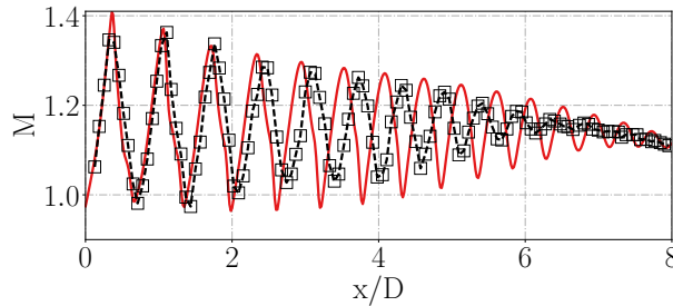
Figure 21: Mach number profile at AXIS. Legends: - \square - LMFA experiment [46] (notched nozzle), — LES
