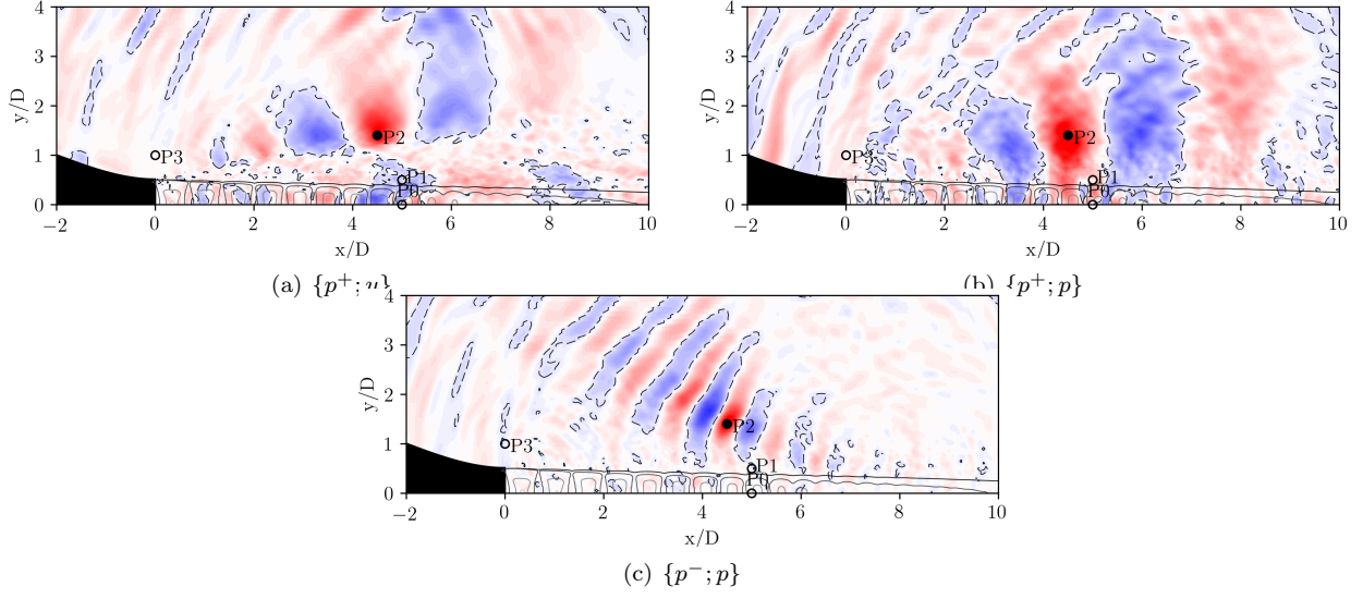
Figure 19: Normalized two-dimensional cross-conditioning maps of (a) \{p^+; u\} , (b) \{p^+; p\} and (c) \{p^-; p\} , where the reference signal is located at P2. The results are normalized by the local standard deviation and are plotted between +1 (red contours) and -1 (blue contours). The dashed contours depict the negative regions. The black solid lines represent the Mach number contours above 1
