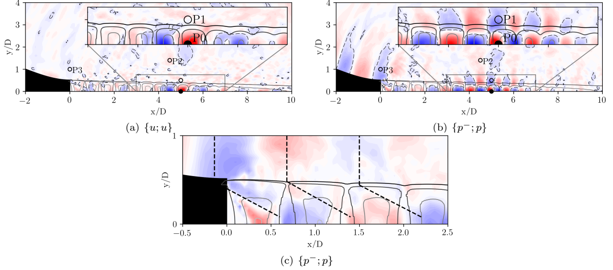
Figure 15: Normalized two-dimensional cross-conditioning maps of (a) \{u; u\} and (b) \{p^-; p\} . The results are normalized by the local standard deviation and are plotted between +1 (red contours) and -1 (blue contours). The dashed contours depict the negative regions. The black solid lines represent the Mach number contours above 1. Figure (c) is a detail of (b) at the nozzle exit where the waves that enter the potential core are depicted by dashed lines
