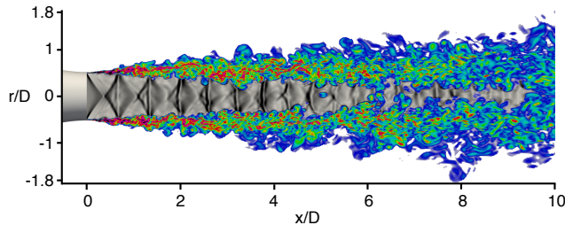
Figure 6: LES of under-expanded jet: magnitude of density gradient (numerical Schlieren, in grey) and vorticity modulus (in color |\Omega| \in [1.8, 320.0] \times 10^4 \text{ s}^{-1} )
