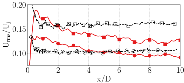
Figure 22: Turbulence levels of the axial ( U_{rms} ) and radial ( V_{rms} ) component of velocity at LIPLINE ( r/D = 0.5 ). Legends: U_{rms} - \square - and V_{rms} - \ominus - from LMFA experiment [46]. U_{rms} - \blacksquare - and V_{rms} - \bullet - from LES
