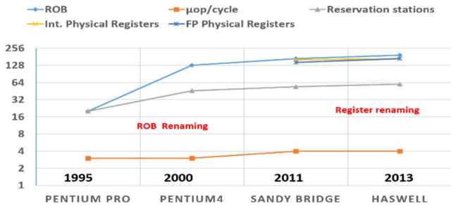
Fig. 8. IPC limits in Intel out-of-order CPUs
