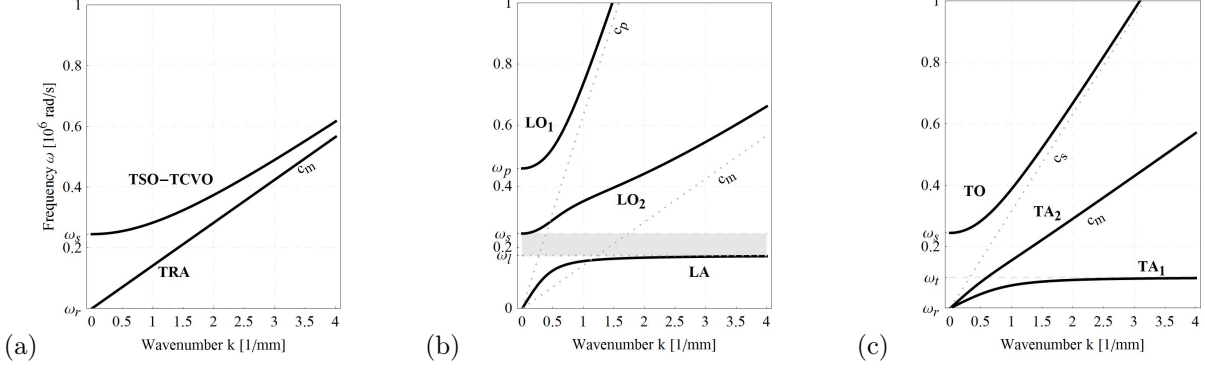
Figure 6: Dispersion relations \omega = \omega(k) for the relaxed micromorphic model with vanishing Cosserat couple modulus \mu_c = 0 : only a partial band gap can be modeled.
