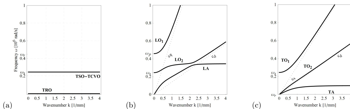
Figure 4: Dispersion relations \omega = \omega(k) for the micromorphic model with \|\text{Div } P\|^2 and vanishing Cosserat couple modulus \mu_c = 0 : no band gap on the longitudinal and transverse waves can be modeled and the uncoupled waves have fixed frequencies.
