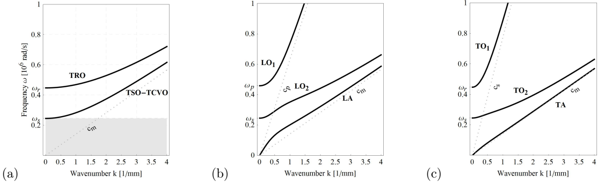
Figure 7: Dispersion relations \omega = \omega(k) for the standard micromorphic model with \|\nabla P\|^2 with non-vanishing Cosserat couple modulus \mu_c > 0 : only a partial band gap can be modeled for uncoupled waves.
