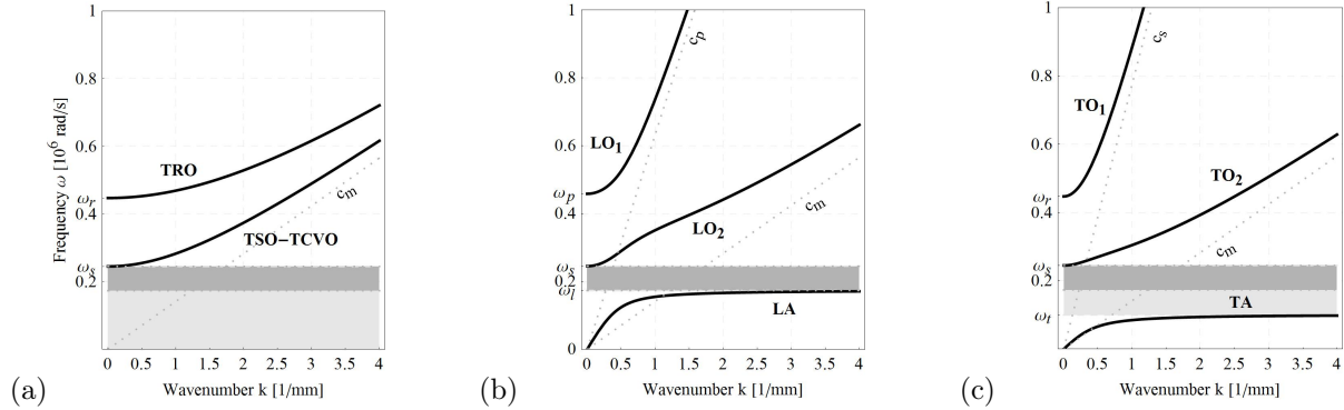
Figure 5: Dispersion relations \omega = \omega(k) for the relaxed micromorphic model with non-vanishing Cosserat couple modulus \mu_c > 0 . Complete frequency band gap is the shaded intersected domain bounded from the maximum between \omega_l and \omega_t and the minimum between \omega_r and \omega_s . The existence of the band gap is related to \mu_c > 0 via the cut-off frequency \omega_r = \sqrt{\frac{2\mu_c}{\eta}} of the uncoupled waves TRO and TO1
