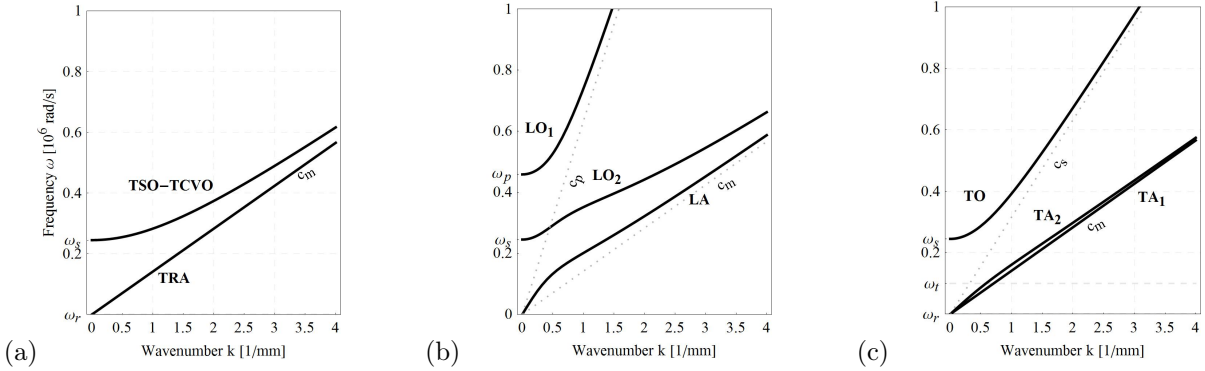
Figure 2: Dispersion relations \omega = \omega(k) for the micromorphic model with \|\text{Div } P\|^2 + \|\text{Curl } P\|^2 and vanishing Cosserat couple modulus \mu_c = 0 : no band gap at all.
