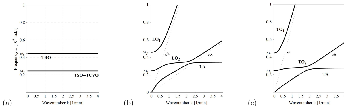
Figure 3: Dispersion relations \omega = \omega(k) for the micromorphic model with \|\text{Div } P\|^2 and non-vanishing Cosserat couple modulus \mu_c > 0 : no band gap on the longitudinal and transverse waves can be modeled and the uncoupled waves have fixed frequencies.
