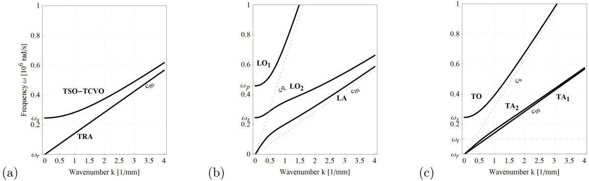
Figure 8: Dispersion relations \omega = \omega(k) for the standard micromorphic model with \|\nabla P\|^2 and vanishing Cosserat couple modulus \mu_c = 0 : no band gap at all.
