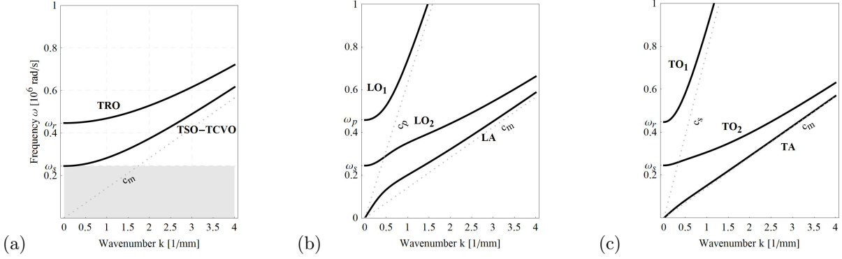
Figure 1: Dispersion relations \omega = \omega(k) for the micromorphic model with \|\text{Div } P\|^2 + \|\text{Curl } P\|^2 and non-vanishing Cosserat couple modulus \mu_c > 0 : only a partial band gap on the uncoupled waves can be modeled.
