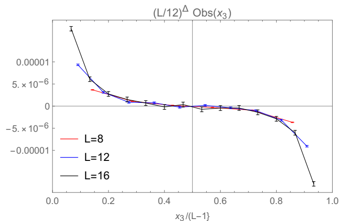
Figure 3. In this plot \Delta = 6 , which is our central value for \Delta_V .
