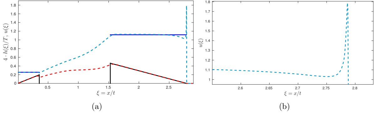
Figure 5. Validation of similarity solution by unsteady simulations. Left panel (a): the exact solution is depicted with solid lines (black — scaled flow height 4 \frac{h(\xi)}{T} , blue — u(\xi) ) and unsteady numerical prediction are shown with dashed lines (red — layer height, blue — horizontal speed). Right panel (b): zoom on the jump in the velocity variable at the flow head.
