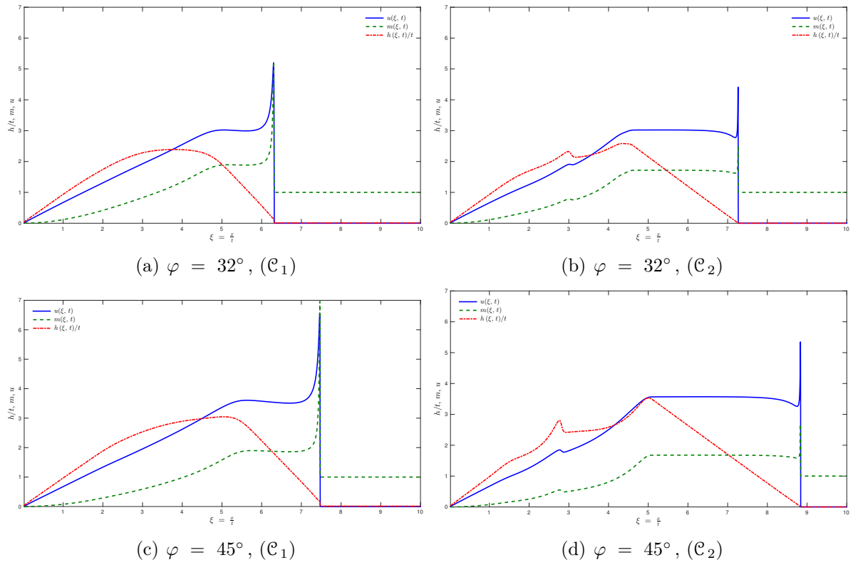
Figure 6. Self-similar profiles emerging from the lock-exchange problem at the final simulation time t = T .
