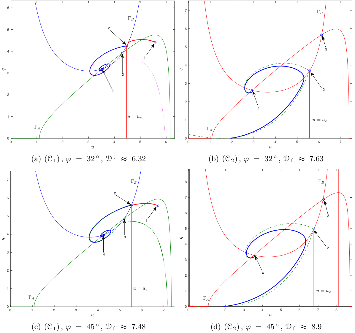
Figure 7. Behaviour of thermal solutions in the phase plane (u, q) for different slopes \alpha = \tan \varphi and different initial conditions (\mathcal{C}_{1,2}) . Trans-critical are shown in panels (a) and (c), while super-critical flows in panels (b) and (d).
