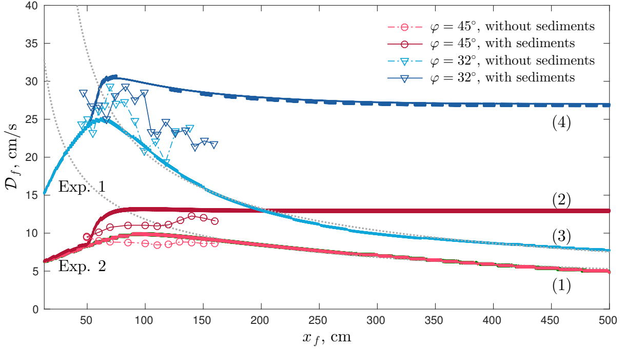
Figure 4. Evolution of the front velocity \mathcal{D}_f of laboratory clouds as a function of downstream distance x_f . Comparison of the predicted flow head velocity (lines without markers) against the experimental results (lines with markers) from RASTELLO & HOPFINGER (2004) [64, Fig. 11]. The upper (lower) group of data corresponds to Experiment 1 (2) from Table 2. Dotted lines show the asymptotic regime \mathcal{D}_f \sim \frac{1}{\sqrt{x_f}} demonstrated in [49].
