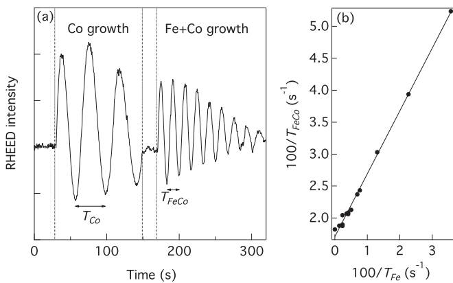
FIG. 1. (a) RHEED intensity oscillations during the growth of, first, Co alone and, second, a FeCo alloy on a Fe(001) buffer layer. (b) Working at a fixed Co growth rate and varying the Fe growth rate leads to a linear variation of the inverse of both periods as in Eq. (2).
