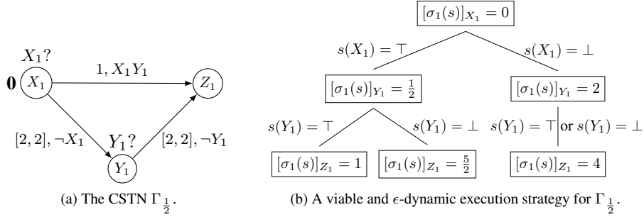
Figure 9: A dynamically-consistent CSTN whose viable and dynamic execution strategies are fractional.
