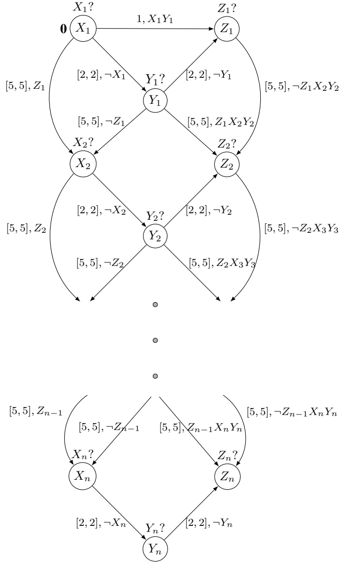
Figure 11: A CSTN \Gamma^n such that \hat{c}(\Gamma^n) = 2^{-\Omega(|P^n|)} .
