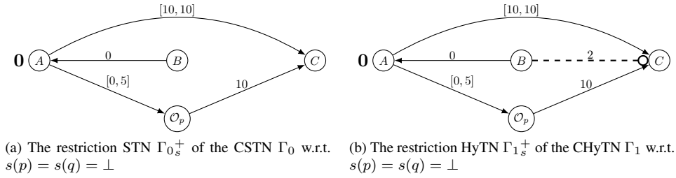
Figure 4: The restriction \Gamma_{0_s^+} (a), and the restriction \Gamma_{1_s^+} (b), w.r.t. the scenario s(p) = s(q) = \perp
