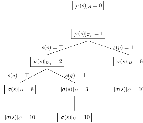
Figure 5: A tree-like representation of a dynamic execution strategy \sigma for the CHyTN \Gamma_1 of Fig. 3b, where s denotes scenarios and [\sigma(s)]_X is the corresponding schedule.
