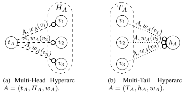
Figure 1: Multi-Head and Multi-Tail Hyperarcs.
