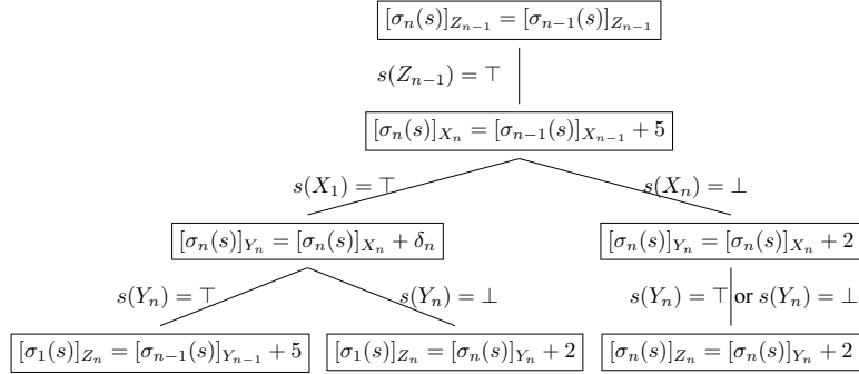
Figure 13: A viable and dynamic execution strategy for the inductive step n - 1 \rightsquigarrow n when s(Z_{n-1}) = \top .
