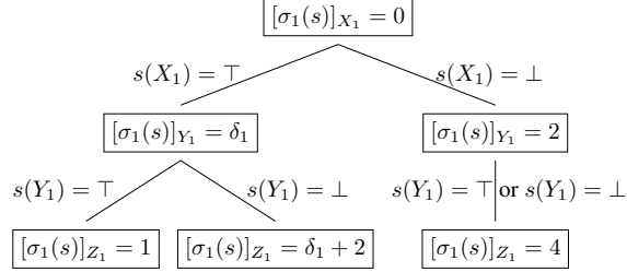
Figure 12: A viable and dynamic execution strategy for the base case n = 1 .
