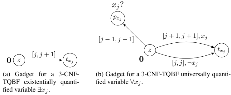
Figure 7: Gadgets for quantified variables used in the reduction from 3-CNF-TQBF to General-CHyTN-DC.
