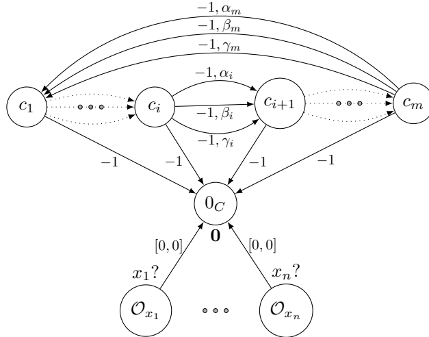
Figure 6: The CSTN N^\varphi where \varphi(x_1, \dots, x_n) = \bigwedge_{i=1}^m c_i for c_i = (\alpha_i \vee \beta_i \vee \gamma_i) .
