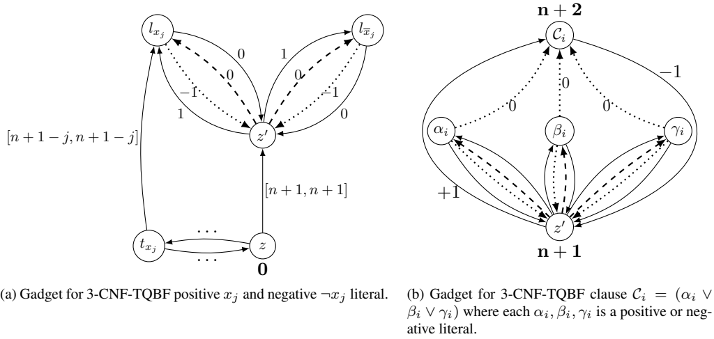
Figure 8: Gadgets used for variables and clauses in the reduction from 3-CNF-TQBF to General-CHyTN-DC.
