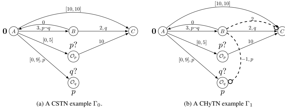
Figure 3: An example CSTN (a), and an example CHyTN (b).
