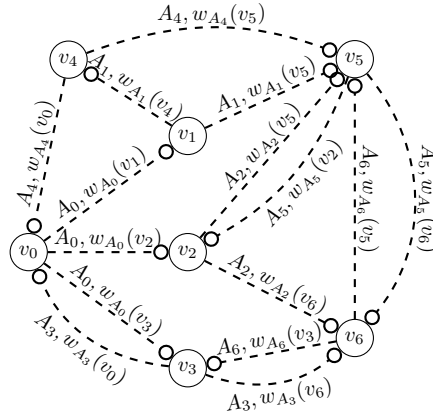
Figure 2: A Cycle (S, \mathcal{C}) , where S = \{v_0, \dots, v_6\} and \mathcal{C} = \{A_0, \dots, A_6\} .
