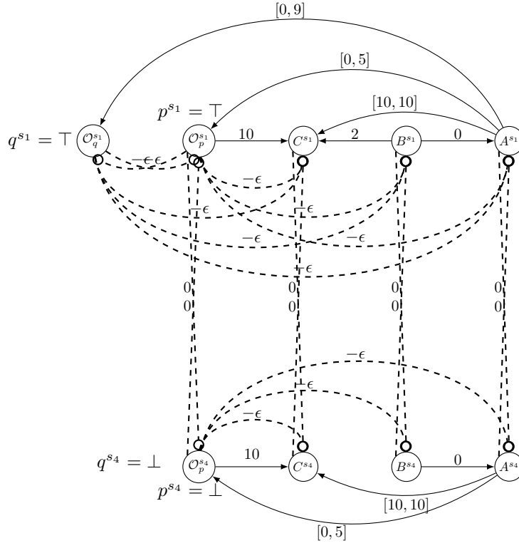
Figure 10: An excerpt of the HyTN \mathcal{H}_\epsilon(\Gamma_0) corresponding to the CSTN \Gamma_0 of Fig. 3a, in which two scenarios, s_1 and s_4 , are considered.
