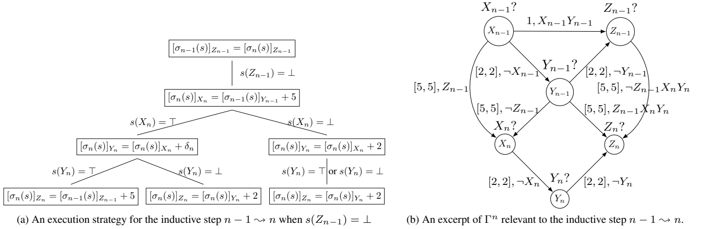
Figure 14: The inductive step n-1 \rightsquigarrow n when s(Z_{n-1}) = \perp .
