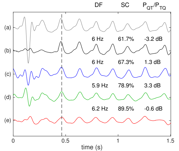
Fig. 4. Experiments on real AF ECG data: atrial signal estimation results. (a) Original single-beat ECG record, precordial lead V1. (b) AA estimated by the ASVC method of [16]. Bottom plots: AA estimated by BTD with R = 12 block terms and matrix factor ranks L = \hat{L}_{PAC} = 17 (c), L = \hat{L}_{MDL} = 48 (d), and L = \hat{L}_{AIC} = 95 (e). Numerical values represent the dominant frequency (DF), spectral concentration (SC) and QT-to-TQ segment power ratio ( P_{QT}/P_{TQ} ) of the different signal estimates.
