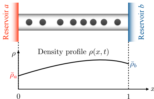
FIG. 1. A schematic diagram of a driven diffusive system with open boundaries.
