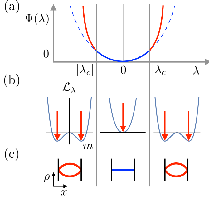
FIG. 2. (a) A schematic illustration of the scaled CGF \Psi(\lambda) exhibiting second-order DPTs associated with particle-hole symmetry breaking. The branch dominated by the symmetric (symmetry-breaking) profile(s) is marked with solid blue (red) lines. The dashed blue lines indicate the action of the symmetric profile when it is no longer optimal. (b) The Landau theory \mathcal{L}_\lambda(m) in each regime of \lambda . (c) The optimal density profile(s) in each regime of \lambda .
