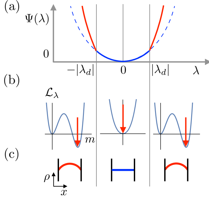
FIG. 3. (a) A schematic illustration of the scaled CGF \Psi(\lambda) exhibiting first-order DPTs for \bar{D}\bar{\sigma}^{(3)} > 3\bar{D}'\bar{\sigma}'' . The branch dominated by the flat (non-flat) profiles is marked with solid blue (red) lines. The dashed blue lines indicate the action of the flat profile when it is no longer optimal. (b) The Landau theory \mathcal{L}_\lambda(m) and (c) the optimal density profiles in each regime of \lambda .
