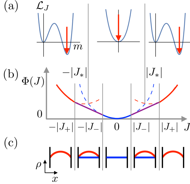
FIG. 6. (a) The Landau theory \mathcal{L}_J(m) , obtained by assuming the additivity principle, in different regimes of J demarcated by J = \pm|J_*| . (b) A schematic illustration of the LDF \Phi(J) exhibiting first-order DPTs. The branch dominated by the flat (non-flat) profile(s) is marked with solid blue (red) lines, and the coexistence regimes of both profiles are marked with solid purple lines. The dashed blue (red) lines indicate the action of the flat (non-flat) profile when it occupies the entire history. (c) The optimal density profiles in each regime of \lambda .
