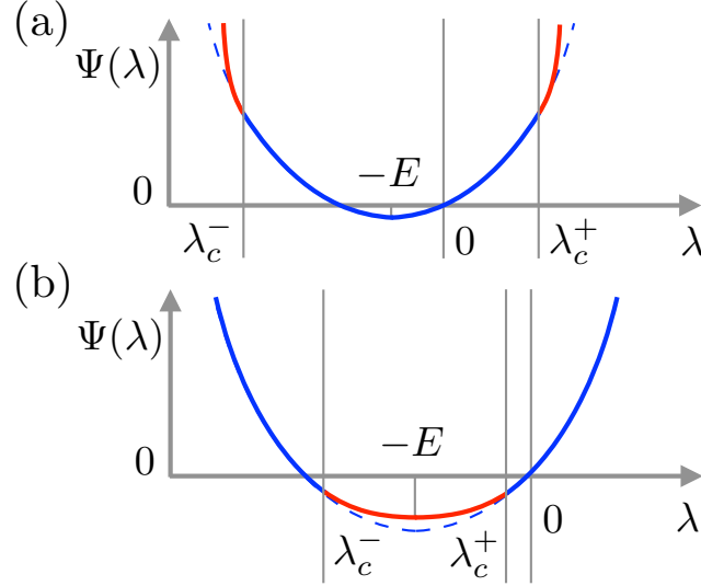
FIG. 4. (a) A schematic illustration of the scaled CGF \Psi(\lambda) exhibiting symmetry-breaking DPTs when E > 0 and \bar{\sigma}'' > 0 . The branch dominated by the symmetric (symmetry-breaking) profile(s) is marked with solid blue (red) lines. The dashed blue lines indicate the action of the symmetric profile when it is no longer dominant. (b) The behavior of \Psi(\lambda) when E > 0 and \bar{\sigma}'' < 0 .
