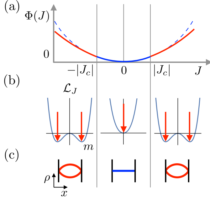
FIG. 5. (a) A schematic illustration of the LDF \Phi(J) exhibiting second-order DPTs associated with particle–hole symmetry breaking. The branch dominated by the symmetric (symmetry-breaking) profile(s) is marked with solid blue (red) lines. The dashed blue lines indicate the action of the symmetric profile when it is no longer dominant. (b) The Landau theory \mathcal{L}_J(m) in each regime of \lambda . (c) The optimal density profiles in each regime of \lambda .
