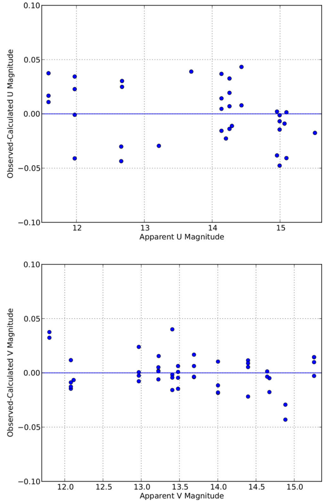
Figure 1. Comparison of our calibrated magnitudes with the ones obtained by Landolt (1992). The upper panel shows the dispersion in the U band for Night 1 – expected to be less good than the lower panel – the dispersion in the V band for Night 6.
