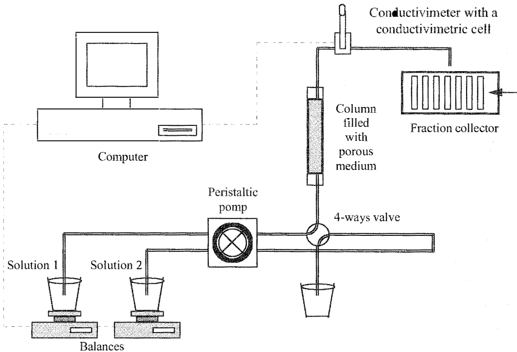
Figure 1. Experimental set-up.
