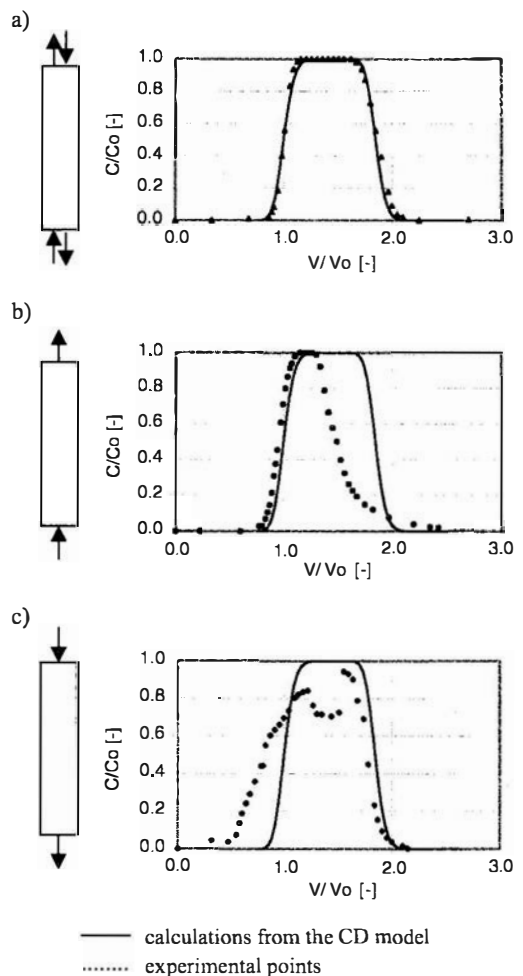
Figure 2. Experimental and calculated breakthrough curves during: a) bead size: d_1 = 1 mm; stable flow, b) bead size: d_2 = 4 mm; unstable ascending flow, c) bead size: d_2 = 4 mm; unstable descending flow.
