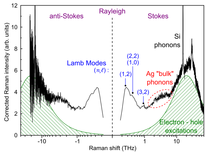
FIG. 4. (Color online) Stokes and anti-Stokes Raman spectra of a SiO 2 (1 \mu\text{m} )/Si sample obtained by implanting 4 \times 10^{16} Ag + ions/cm 2 with a kinetic energy of 190 keV. The intensity has been corrected by the Bose population factor. The hatched area is delimited by a fit of the theoretical single-particle response. Note the unusual log scale adopted for the Raman shift.
