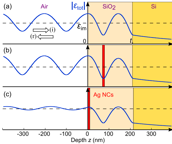
FIG. 3. (Color online) Variation vs depth of the amplitude of the total (incident i + reflected r ) electric field |\mathcal{E}_{\text{tot}}| = |\mathcal{E}_i + \mathcal{E}_r| : (a) without Ag NCs, (b) with a plane of Ag NCs located at a node of the electric field into the dielectric layer, and (c) with this plane located at an antinode of the electric field near the dielectric/air interface. The wavelength in vacuum is chosen at 413 nm in coincidence with the plasmon frequency, the thickness of the layer is 210 nm, the incidence is normal, the diameter of the Ag NCs is 5 nm, and the amount of silver equals 5 \times 10^{16} atoms/cm 2 .
