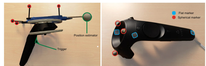
Figure 3. Controller with estimation attached to it (left). Controller used to align Optitrack and HTC Vive spaces, markers placed to easily identify origin and orientation of the controller (right).
