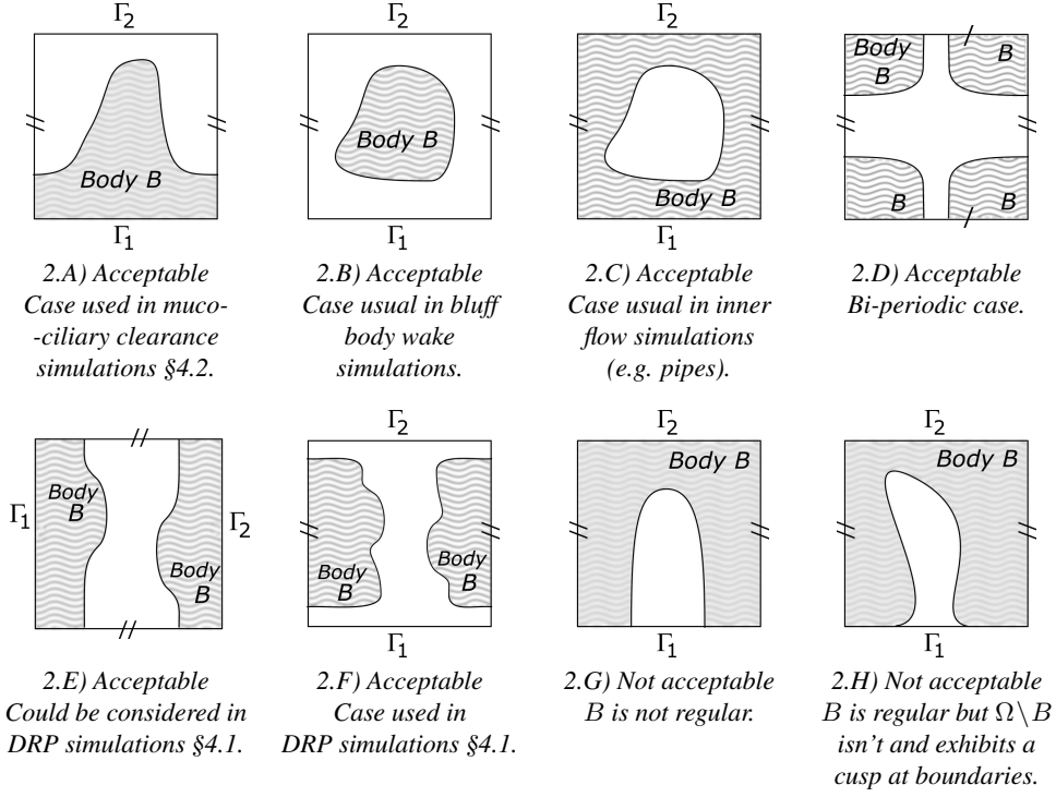
Figure 2: Acceptable cases of domains B for the C^k -bi-regularity property introduced in definition 1.2.
