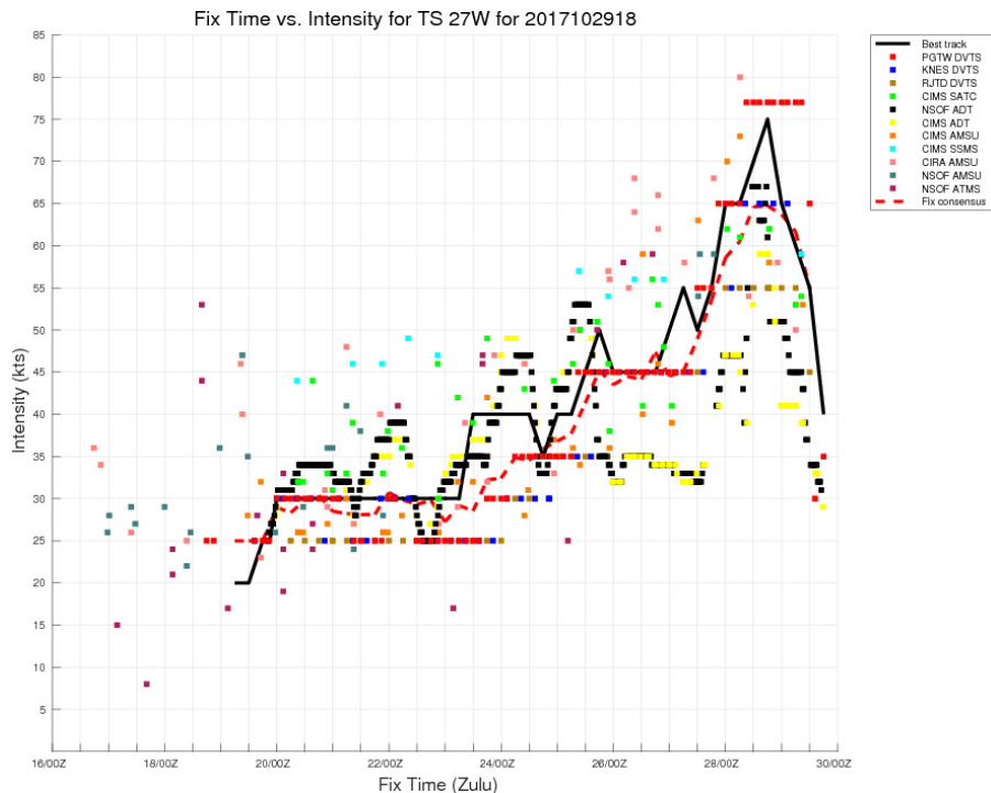
Figure 10. Example intensity time history for TC 27W (2017) showing the intensity analysis estimates currently available to the JTWC forecaster. All estimates listed in the label from “CIMS SATC” (CIMSS SATCON) down are based on automated analysis techniques. These estimates facilitate intensity analysis in open-ocean and near-landfall scenarios alike. Further refinements to these techniques will increase intensity analysis accuracy.
