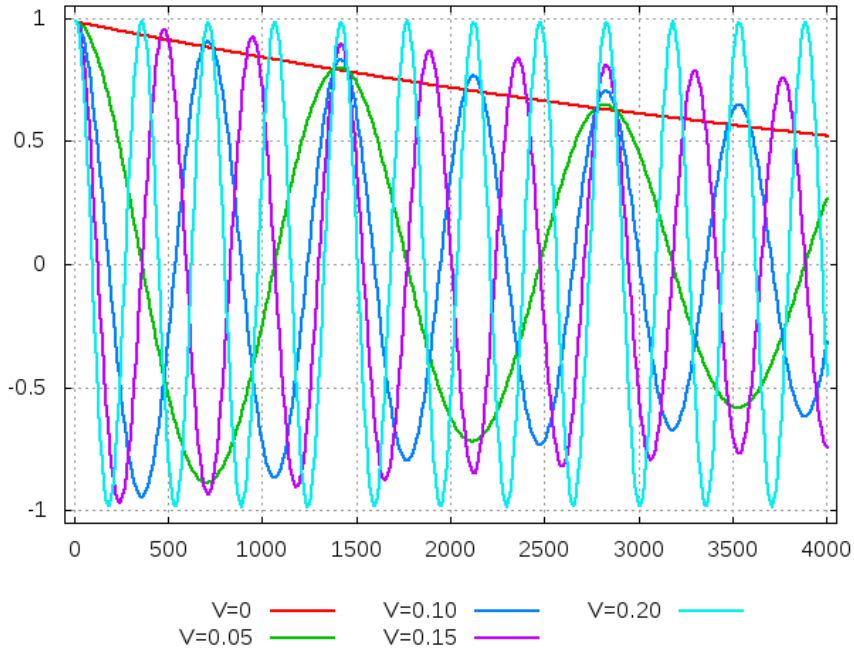
Figure 1: Time evolution of the correlation function A(t)/A(0) versus discrete time between an initial transverse wave (of vector (3k_0, 2k_0) where k_0 = \frac{2\pi}{191} ) and its later state for five different values of the mean velocity V . Square of 191 \times 191 nodes and periodic boundary conditions. When V grows, the dissipation of the waves is reduced.
