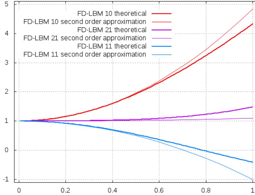
Figure 4: Relative shear viscosity (normalized by \nu_0 ) for the nine point stencil versus wave vector modulus k . Solid curves from dispersion equation, thin solid curves from hyperviscosity, squares from actual simulation. Top curves for wave vector along X axis, middle curves for wave vector along \{2,1\} direction and lower curves for wave vector along the \{1,1\} direction. No experimental data due to linear instability at least in the \{1,1\} direction.
