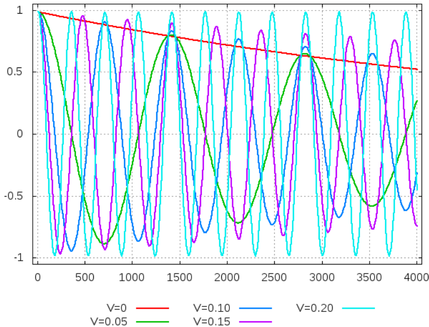
Figure 1: Time evolution of the correlation function A(t)/A(0) versus discrete time between an initial transverse wave (of vector (3k_0, 2k_0) where k_0 = \frac{2\pi}{191} ) and its later state for five different values of the mean velocity V . Square of 191 \times 191 nodes and periodic boundary conditions. When V grows, the dissipation of the waves is reduced.
