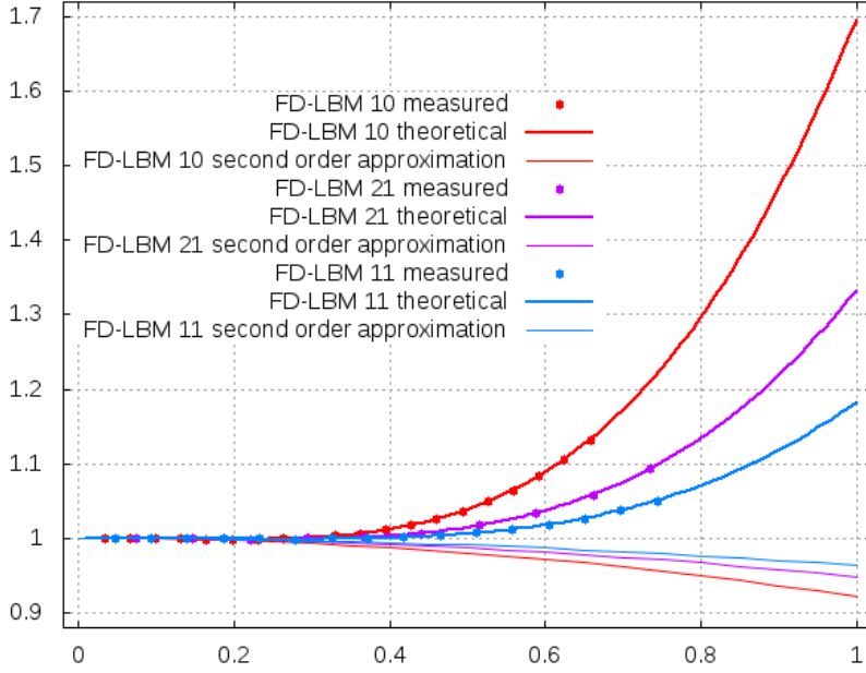
Figure 3: Relative shear viscosity (normalized by \nu_0 ) for the five point stencil versus wave vector modulus k . Solid curves from dispersion equation, thin solid curves from hyperviscosity, discrete points from actual simulation. Top curves for wave vector along X axis \{1,0\} , middle curves for wave vector along \{2,1\} direction and lower curves for wave vector along the \{1,1\} direction.
