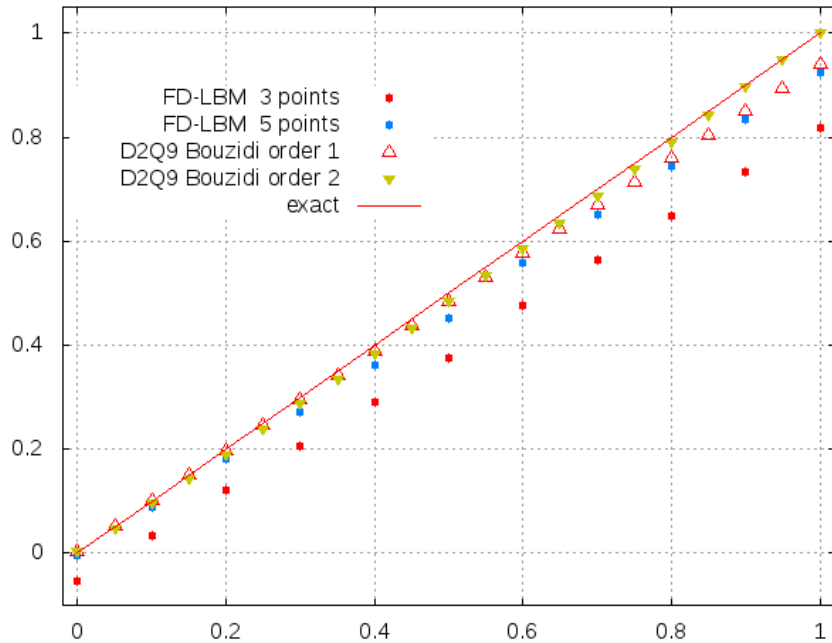
Figure 6: Boundary conditions for a Poiseuille flow. Numerical location of the zero of velocity versus the imposed value \xi of the boundary. In the transverse direction, the computational domain is composed by the interval [1 - \xi, 15 + \xi] where \xi is the abscissa of the figure. The result is the location of the zero velocity value measured from a least square fit of the velocity profile. The result with the five points difference scheme is of good quality, comparable to what is obtained with the classical D2Q9 usual LBM scheme with first order extrapolation with the Bouzidi et al. algorithm. Observe that with a simple “bounce-back” boundary conditions, the result would be a horizontal line at y = 0.5 .
