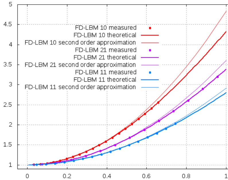
Figure 2: Relative shear viscosity (normalized by \nu_0 ) for the three point stencil versus wave vector modulus k . Solid curves from dispersion equation, thin solid curves from hyperviscosity, discrete points from actual simulation. Top curves for wave vector along X axis \{1,0\} , middle curves for wave vector along \{2,1\} direction and lower curves for wave vector along the \{1,1\} direction.
