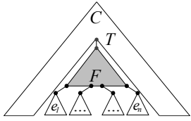
Figure 4: A fragment within a larger QIR term
