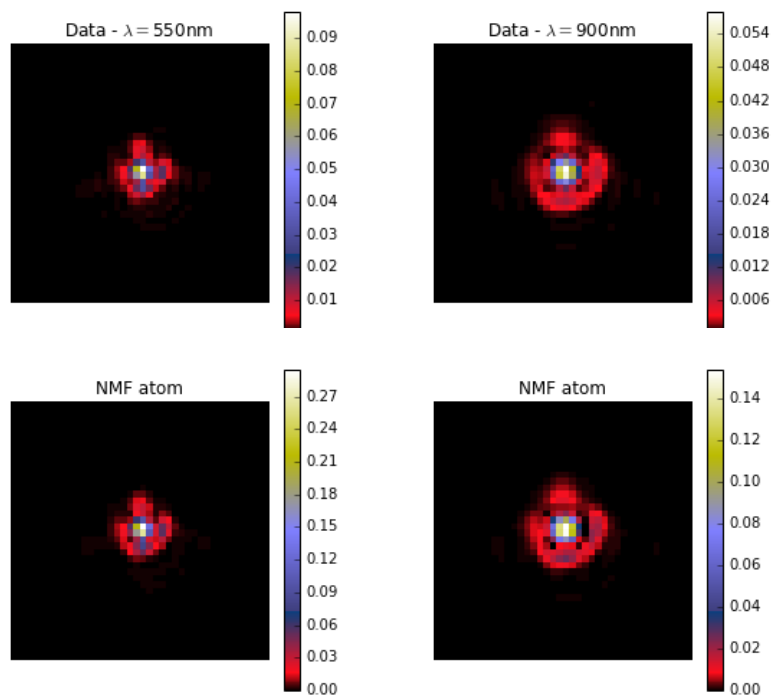
Figure E.1: Extreme wavelength PSFs in the dataset and atoms learned from NMF. See Figure 7 for those learned using our method.
