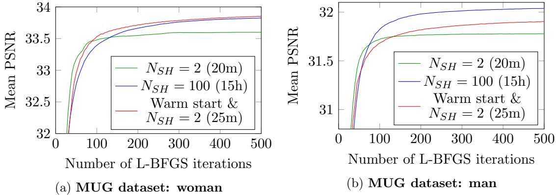
Figure 4: Evolution of the mean PSNR of the reconstructions per L-BFGS iteration, for 3 configurations, on 2 datasets. The KL loss was used for this experiment. We see that the warm start yields better reconstructions with the same number of Sinkhorn iterations ( N_{SH} ), in roughly the same time.
