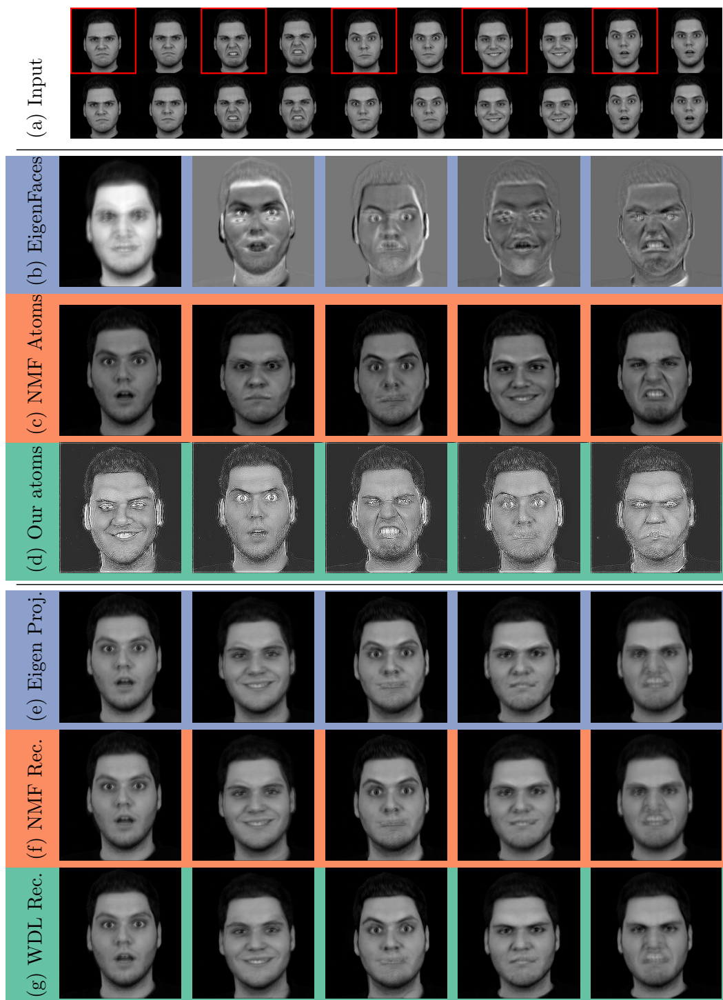
Figure E.2: Similarly to Figure 11 , we compare our method to the Eigenfaces [71] approach and Non-negative Matrix Factorization as a tool to represent faces on a low dimensional space.
