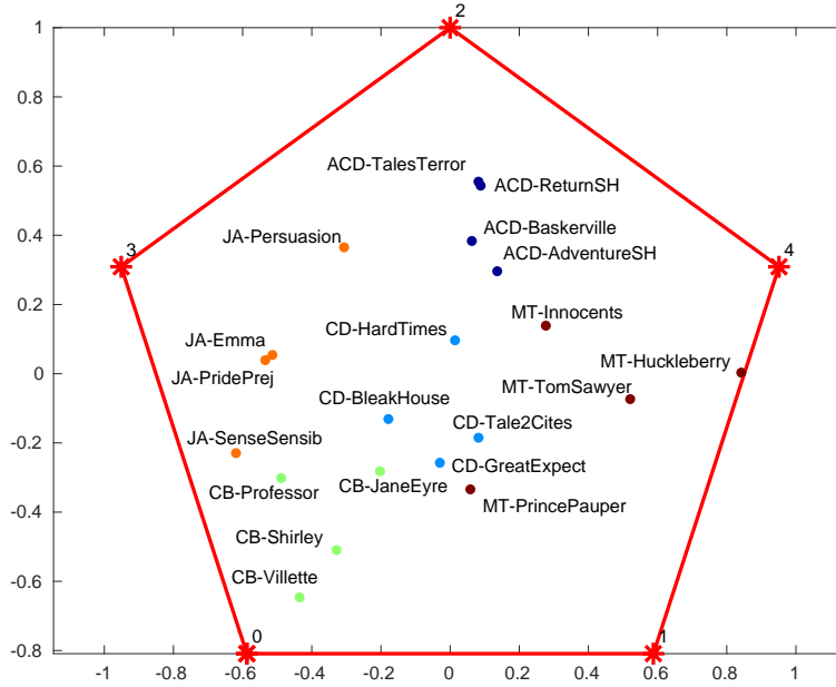
Figure 14: Book classification: using our algorithm, we look at word histograms of novels, and learn 5 atoms in a sample of 20 books by 5 authors. We plot each book according to its barycentric coordinates with regard to the learned atoms. Our algorithm successfully classifies books by author.
