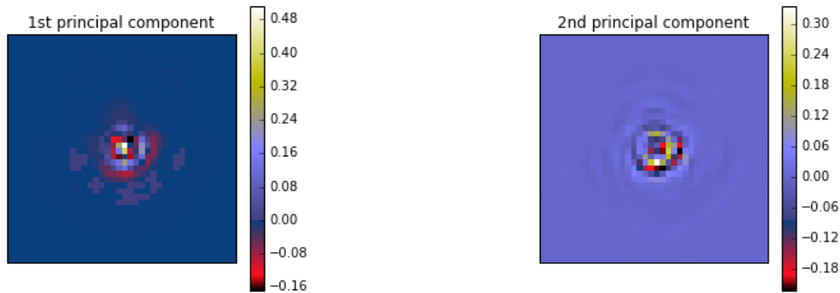
Figure 8: PCA-learned components.
