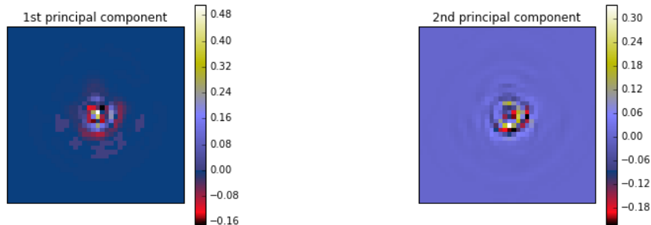
Figure 8: PCA-learned components.
