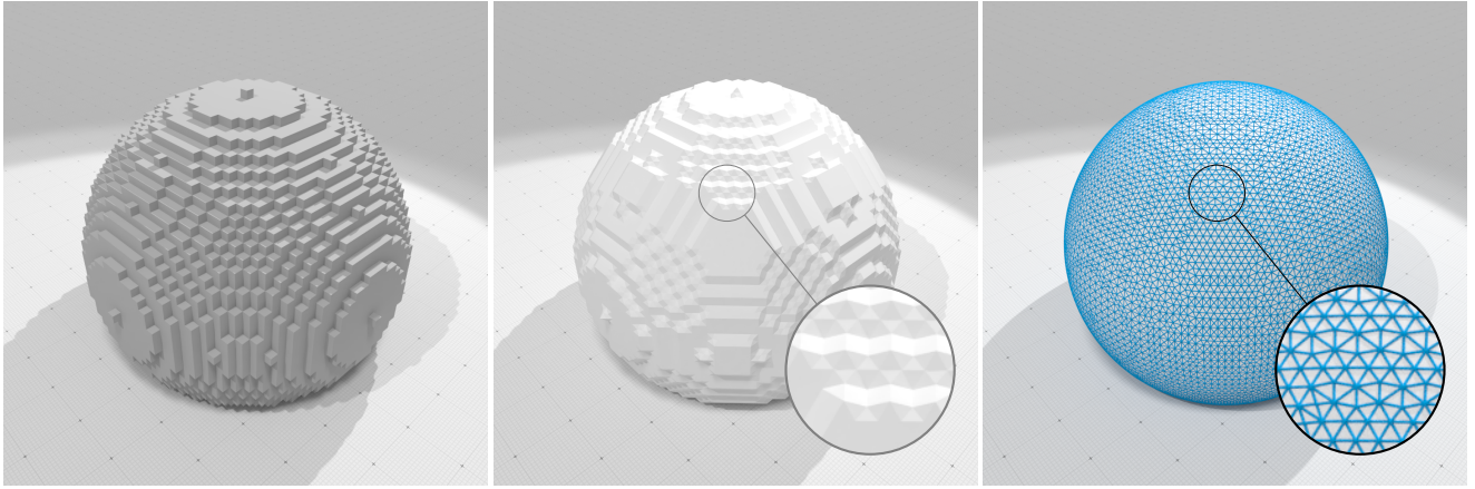
Fig. 7 Discrete settings used for the comparison between various Laplace–Beltrami operators. The unit ball S^3 is discretized using the Gauss digitization process. The left image is the digital surface \partial_h S^3 where we compute L_h and \mathcal{L}_{COMBI} . The image in the center is the marching-cubes associated with the digital surface where we compute \mathcal{L}_{MESH} , \mathcal{L}_{R-LOC} and \mathcal{L}_{COT} . Finally, the right image represents the projection of the marching-cubes on \partial S^3 where \mathcal{L}_{MESH}^P , \mathcal{L}_{R-LOC}^P and \mathcal{L}_{COT}^P are computed.
