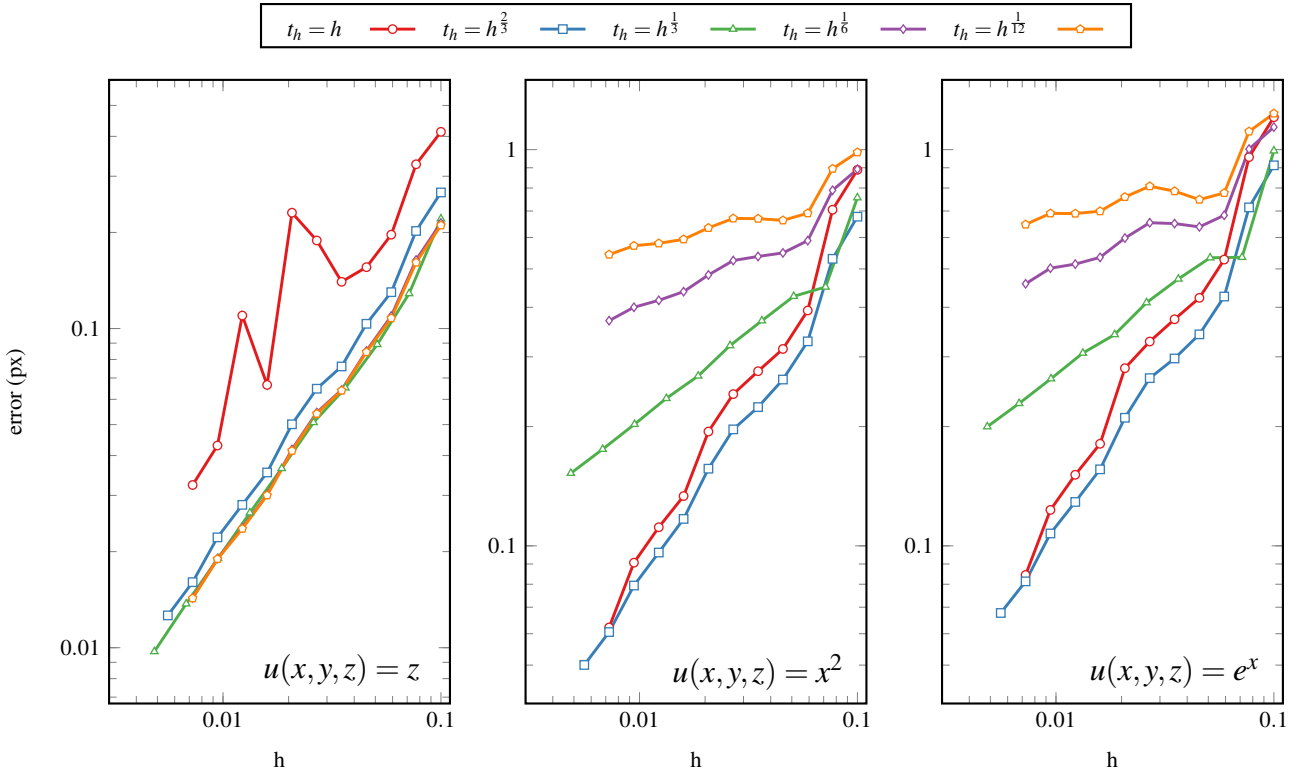
Fig. 8 Consistency results between \Delta and L_h for the l_\infty norm are shown for various functions on the unit sphere \partial \mathbb{S}^3 . We use either t_h = h in red, t_h = h^{2/3} in blue, t_h = h^{1/3} in green, t_h = h^{1/6} in purple and t_h = h^{1/12} in orange.
