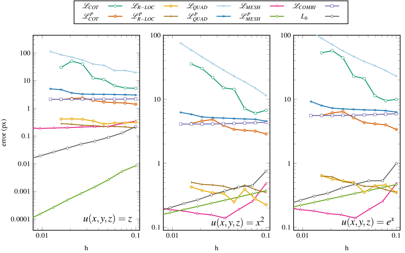
Fig. 9 Multigrad convergence graphs for various functions on \partial S^3 , the unit sphere. l_\infty is displayed for \mathcal{L}_{COT} , \mathcal{L}_{COT}^P , \mathcal{L}_{COMBI} , \mathcal{L}_{MESH} , \mathcal{L}_{MESH}^P , \mathcal{L}_{R-LOC} , \mathcal{L}_{R-LOC}^P , \mathcal{L}_{QUAD} , \mathcal{L}_{QUAD}^P and L_h . Parameters t_h and r are equal to h^{\frac{1}{3}} for all five convolution operators.
