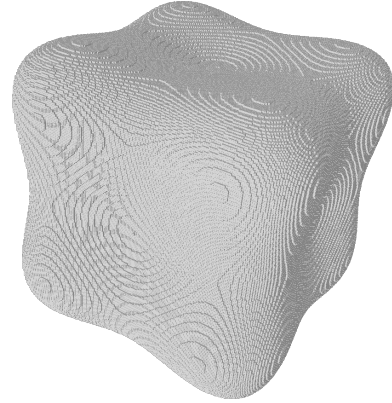
Fig. 10 The digital surface associated to the Goursat equations used to compute mean curvature.
