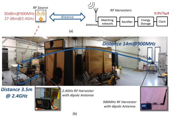
Figure 5. Remote powering of a 0.9V/5μA clock at 900MHz and 2.4GHz: schematic of the scene (a) picture (b)
