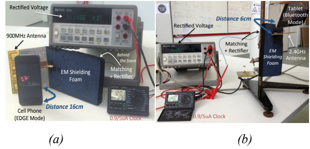
Figure 7: Scavenging scenario of RF energy for clock powering at 900MHz with a cell phone in GSM/EDGE mode (a) at 2.4GHz with a tablet in Bluetooth connection (b)
